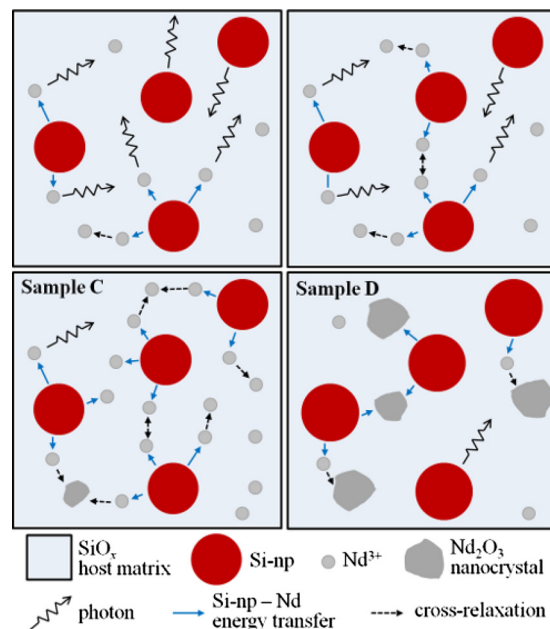
FIG. 8. (Color online) Schematic illustration of a model of the evolution of PL of Si-np \text{Nd}^{3+} ions as function of the Nd concentration.
