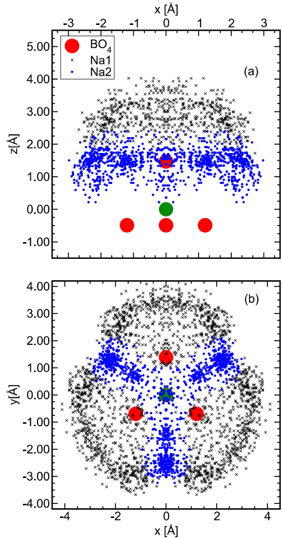
FIG. 7. Distribution of the Na atoms around a BO 4 tetrahedron. a) Top view. Only the Na atoms that are first nearest neighbor of oxygen #1 (the top one) are shown. b) Bottom view. Only the Na atoms that are not nearest neighbor of oxygen #1 (at the center) are shown.
