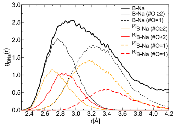
FIG. 5. Decomposition of the 1st peak of the B-Na PDF for the glass according to boron coordination as well as to the number of oxygens that are shared between the B and Na atom.
