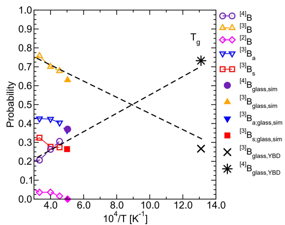
FIG. 2. Temperature dependence in the liquid state of the concentrations of 2-, 3- and 4-fold coordinated borons as well as the ones of the symmetric and asymmetric 3-fold borons, ^{[3]}\text{B}_s and ^{[3]}\text{B}_a respectively. The filled symbols are the corresponding concentrations in the glass generated by the fast quench in the simulation. The dashed lines are the extrapolation of the 3- and 4-fold coordinated borons to low temperatures taking into account that they have to sum up to 100%. The star and cross are the corresponding concentrations as predicted by the YBD model.
