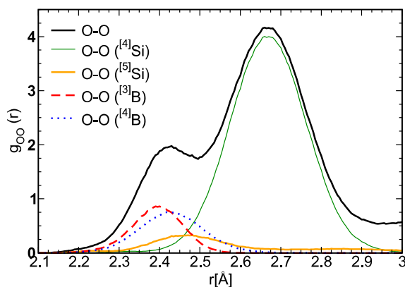
FIG. 4. First peak of the O-O PDF decomposed into contributions of oxygen atoms that are associated with ^{[3]}\text{B} , ^{[4]}\text{B} , and four and five fold coordinated Si.
