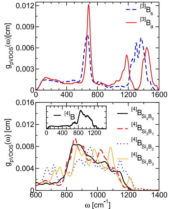
FIG. 12. Partial vibrational of state for boron. (a) Decomposition of the pVDOS for ^{[3]}B into contributions from the symmetric and asymmetric trigonal environments ^{[3]}B_s and ^{[3]}B_a ; (b) Decomposition of the pVDOS for ^{[4]}B into contributions related to different types of second nearest neighbors.
