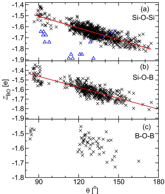
FIG. 15. Dependence of the trace of the Born charge tensors Z_{\text{BO}} for a bridging oxygen atom on its bond angle with the two network formers: (a) Si-O-Si, (b) Si-O-B, and (c) B-O-B. The straight lines are the linear fits with the expressions given by Eqs. (7) and (8). The blue triangles in panel a) are the oxygen triclusters.
