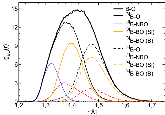
FIG. 3. First peak of the B-O PDF for the glass, decomposed into contributions from ^{[3]}\text{B} and ^{[4]}\text{B} , into oxygen's speciation BO and NBO, as well as according to the second network-former of the bridge B-O-T, for T=Si, B.
