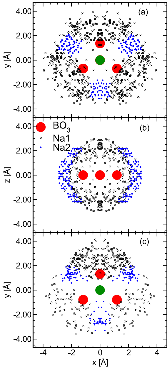
FIG. 6. Distribution of the Na atoms around a BO 3 unit. The crosses and circles show Na atoms that share, respectively, exactly one and two oxygen atom(s) with the central B atoms. a) BO 3 in top view (The oxygen on the top is oxygen #1). b) BO 3 in side view. Only Na atoms that are nearest neighbor to the oxygen atom #1 (at the center) are shown. c) The asymmetric BO 3 unit with two BO and one NBO (oxygen #1, on top).
