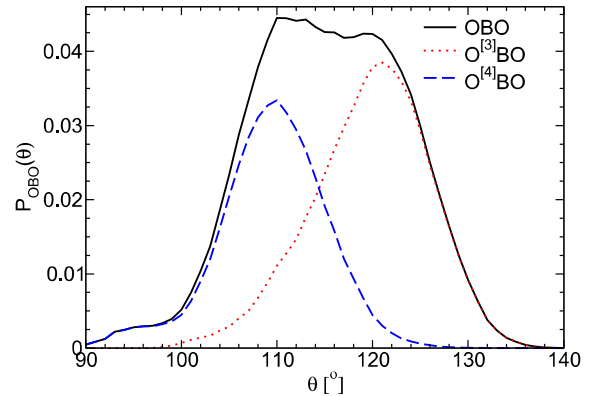
FIG. 9. Distribution of the bond angle O-B-O and its decomposition into O [3] BO and O [4] BO components.
