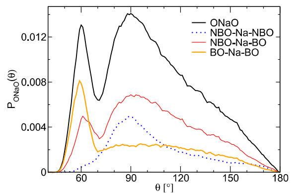
FIG. 10. Distribution of the bond angle O-Na-O and its decomposition for BO and NBO.
