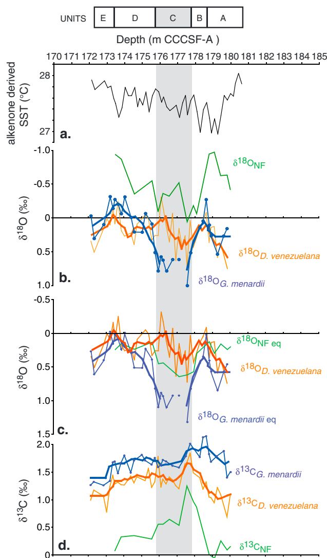
Figure 3. Alkenone-derived calculated (a) SSTs and (b) \delta^{18}\text{O} , and (d) \delta^{13}\text{C} signatures of the planktic foraminifera species G. menardii and D. venezuelana and the calcareous nannofossil separated fraction (NF), respectively, in blue, orange, and green. (c) Vital effect corrected \delta^{18}\text{O} of calcareous nannofossil separated fraction NF (as discussed in the text and Table 2). The vital effect correction of +0.3‰ has been applied to the \delta^{18}\text{O} values of G. menardii , [Bouvier-Soumagnac and Duplessy, 1985] ( D. venezuelana has not been corrected). The thick blue and orange lines correspond respectively to the smoothed curves (5 points) for G. menardii and D. venezuelana obtained using Analyseries 2.0 [Paillard et al., 1996]. The grey-shaded unit C corresponds to the maximum abundance interval of small Dictyococcites spp.
