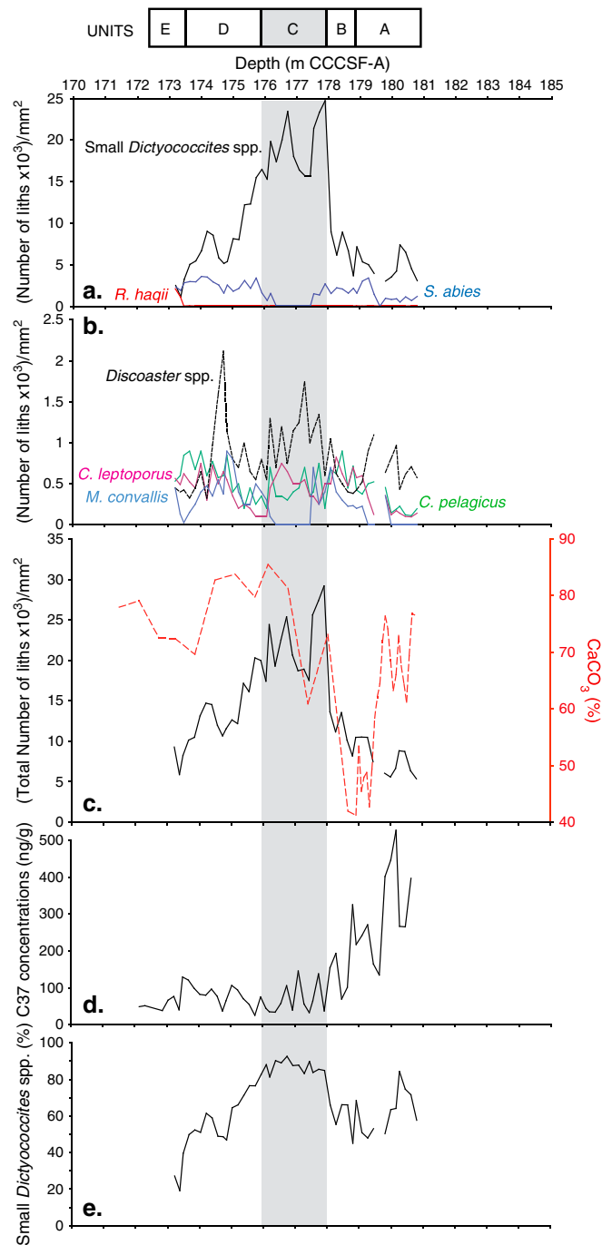
Figure 2. (a and b) Selected calcareous nannofossil absolute abundance record from Site U1338 given per mm 2 . (c) Also reported the CaCO 3 content [Lyle and Backman, 2013] and the absolute total number of nannofossils. (d) The evolution of the C 37 alkenone concentrations in the studied interval. (e) The grey-shaded unit C (see text for explanations) corresponds to the interval of maximum relative abundance of small Dictyococcites spp. in the calcareous nannofossil assemblage.
