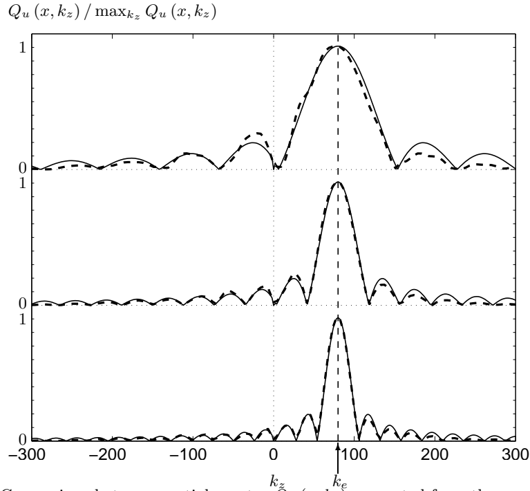
FIGURE 7. Comparison between spatial spectra \hat{Q}_u(x, k_z) computed from the experiments (---) at station x_C = 0.05 m and the theoretical expression (—) computed from (3.4) on the boundary x = 0 , for W = \lambda_e (top), W = 2\lambda_e (middle) and W = 3\lambda_e (bottom).
