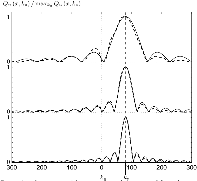
FIGURE 7. Comparison between spatial spectra Q_u(x, k_z) computed from the experiments (---) at station x_C = 0.05 m and the theoretical expression (—) computed from (3.4) on the boundary x = 0 , for W = \lambda_e (top), W = 2\lambda_e (middle) and W = 3\lambda_e (bottom).
