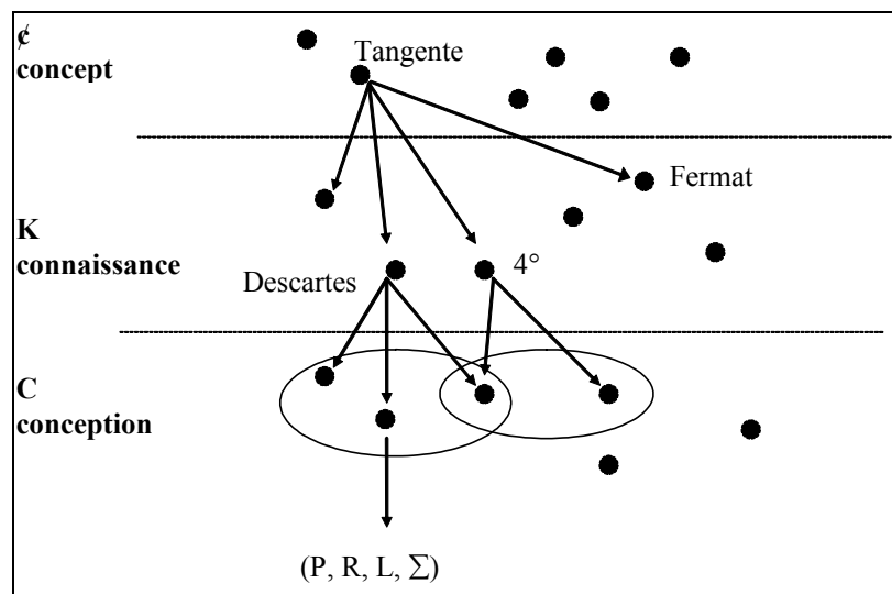
Figure 19. cK \phi
