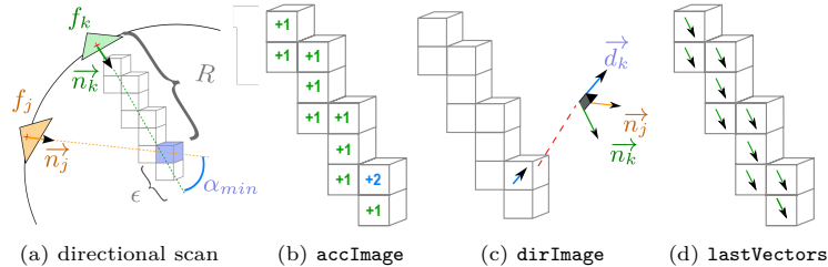
Fig. 3. Illustration of Algorithm 1, which builds an accumulation image whose peaks match the centerline of the tubular shape.
