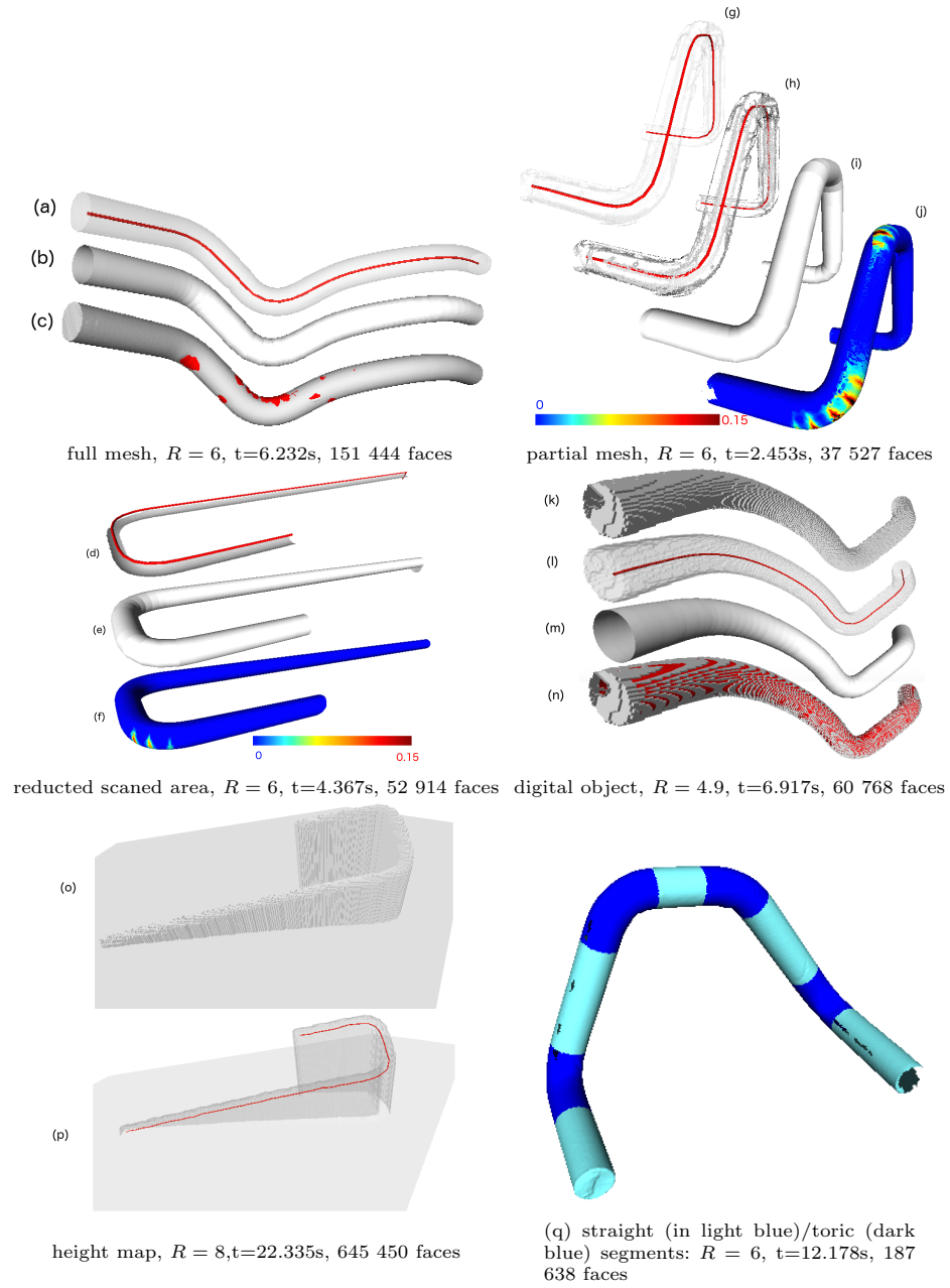
Fig. 8. Result of reconstruction from various input data types. Images (a,g,i,p) show the center line by transparency through the input surface, (k) and (o) are some input surfaces. (b,i,e,m) images are the reconstructed tubes built from the center lines. Images (j) and (f) show the local squared distance error between the reconstructed tube and the input shape and (q) illustrates the decomposition into rectilinear and toric parts. For all experiments, the tracking parameter and epsilon were set respectively to R and 0.001. Running times correspond to executions on a 2,5 GHz Intel Core i7 MacOS computer.
