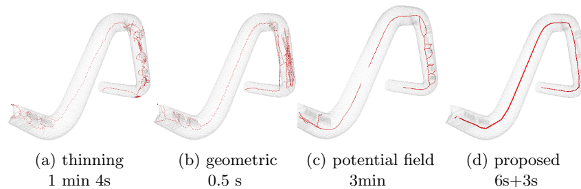
Fig. 2. Skeleton extraction from three different methods presented in [6] with the implementation given by the authors. Our method is presented on the right.
