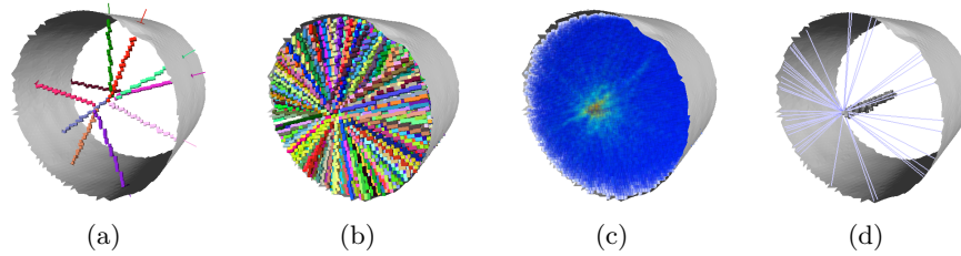
Fig. 4. Illustration of accumulation images generated from surface normal vectors. Image (a) (resp. (b)) illustrates some (resp. all) scanning directions defined from mesh triangles. Image (c) illustrates the values obtained in the 3D accumulation image and (d) shows some voxels having accumulation score upper than a given threshold. In the last image we also display the set of faces contributing to the accumulation score.
