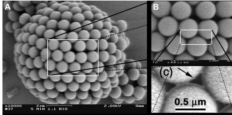
Figure 9. A colloidosome is a spherical shape made of colloids (polystyren molecules here), which is described by Thomson’s model. This model consists in minimizing the interaction |x|^{-s} for particles on the sphere S^2 \subset \mathbb{R}^3 . Scanning microscope picture, from [66]. © AAAS.
