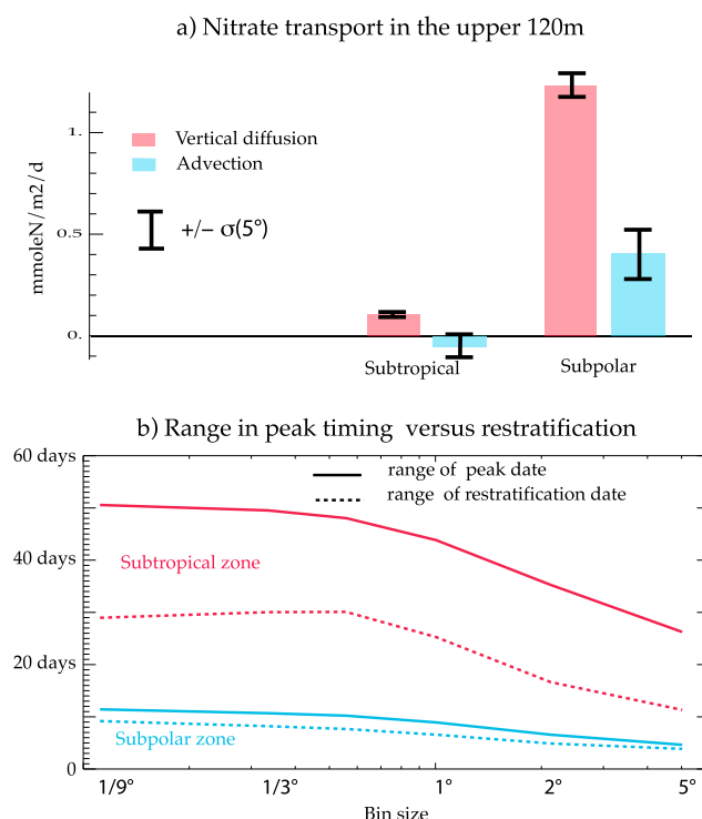
Figure 4. (a) Mean (color bars) \pm \sigma (black horizontal lines) of the annual advective (blue) and diffusive (red) sources of nitrate into the upper 120 m, binned at 5^\circ and averaged over the subtropical and subpolar zones shown in Figure 1a. (b) Range in bloom peak timing (reported from Figure 3b) against bin size, compared with the range in the restratification date (dashed line, defined as the date at which the mixed layer depth has shoaled above 50 m).
