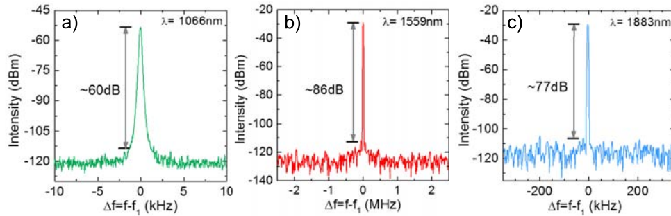
Figure 10. RF spectrum measured around the fundamental repetition rate: (a) f_1 = 16.37 \text{ MHz} , (b) f_1 = 27.4 \text{ MHz} , (c) f_1 = 17.82 \text{ MHz} showing peak to pedestal extinction ratios >60 \text{ dB} in all three wavelengths.
