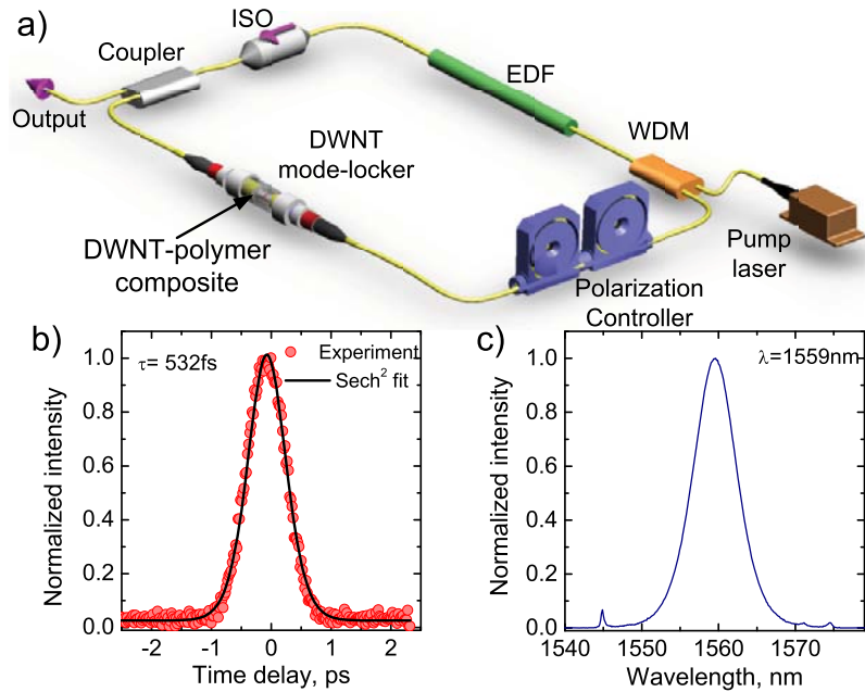
Figure 8. (a) Laser setup at 1.5 \mu\text{m} . EDF, erbium-doped fiber; WDM, wavelength division multiplexer. (b) Second harmonic generation autocorrelation trace of mode-locked pulses at 1.5 \mu\text{m} . (c) Output spectrum.
