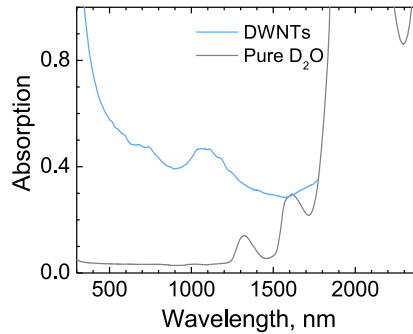
Figure 2. Absorption spectrum of DWNTs dispersed in \text{D}_2\text{O} in the 300 – 1800 nm range. The contribution from \text{D}_2\text{O} is subtracted. Spectrum of \text{D}_2\text{O} is also presented.
