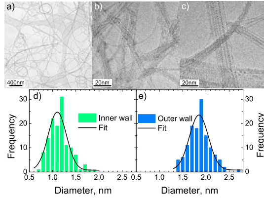
Figure 1. (a–c) Representative TEM images of the purified DWNTs. Inner wall (d) and outer wall (e) diameter distributions as measured from the TEM images shows a mean inner and outer diameter of 1.1 and 1.8 nm, respectively.
