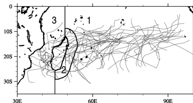
Figure 1. Tracks of the 70 systems from cyclone seasons 2005/2006 to 2012/2013 at intensities of moderate tropical storm, strong tropical storm, tropical cyclone, and intense tropical cyclone. The thick black lines delimit the three subregions considered: 1—open ocean, 2—region near the eastern coast of Madagascar (to 400 km offshore), and 3—Mozambique Channel.
