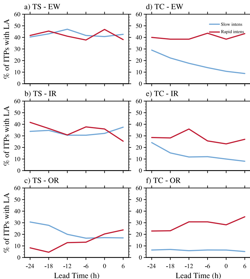
Figure 5. Percentage of ITPs with lightning activity relative to the lead time from intensification (−24h,...,0,...,+6h) for (a–c) TS cases and (d–f) TC cases over the open ocean. Figures 5a and 5d correspond to the eyewall region (EW), Figures 5b and 5e to the inner rainbands region (IR), and Figures 5c and 5f to the outer rainband region (OR). Two thresholds are used for the rate of intensification: 0 < \Delta v_{\max} < 6.6 \text{ kt (6 h)}^{-1} (blue curves) and \Delta v_{\max} \geq 6.6 \text{ kt (6 h)}^{-1} (red curves).
