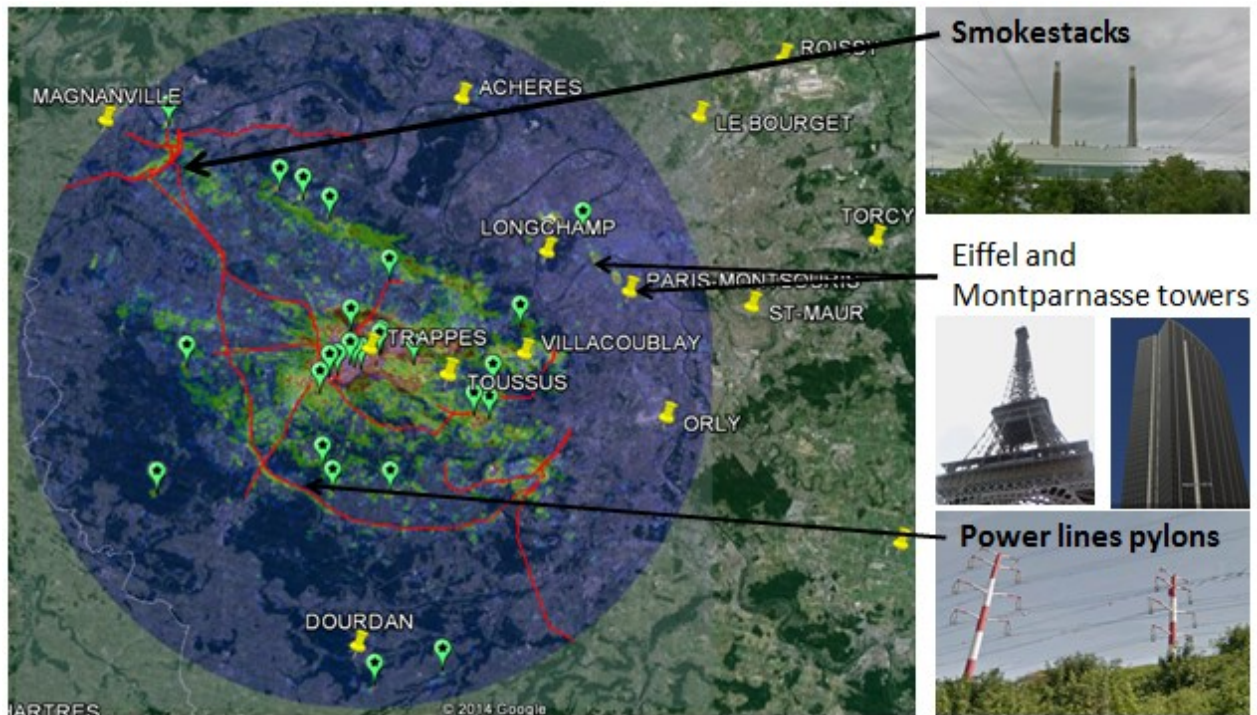
Fig. 1: Reflectivity around Trappes radar at 0.4° elevation angle projected on google maps. Red lines represent power lines. Green points represent other identified ground echoes such as antenna, water tower or buildings. Yellow icons represent Automatic Weather Stations
