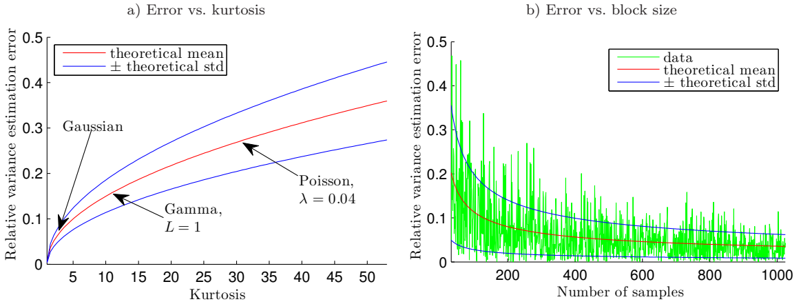
Figure 6. a) Evolution of the expected value and standard deviation of the relative error of the variance estimator as a function of the kurtosis \beta_2 for a size of block N = 16 \times 16 , and b) Evolution of the expected value and standard deviation of the relative variance estimation error as a function of the block size for an additive white Gaussian noise.
