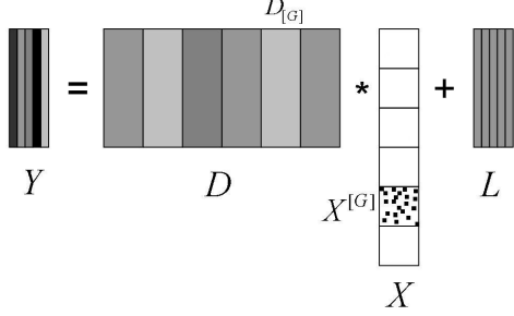
Fig. 3. Pictorial illustration of the constraint in the C-HiSLR.
