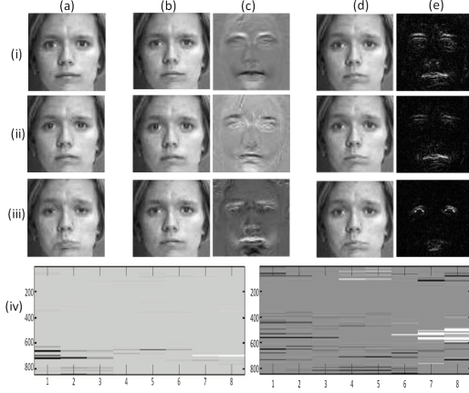
Fig. 4. Effect of group sparsity. \tau_{trn} = 8 . (a) is the test input Y . (b)(c) are recovered L and DX , given by C-HiSLR which correctly classifies (a) as contempt . (d)(e) are recovery results given by SLR which mis-classifies (a) as sadness. (i),(ii),(iii) denote results of frame #1, #4, #8 respectively, whereas (iv) displays the recovered X (left for C-HiSLR and right for SLR). X given by C-HiSLR is group-sparse as we expected.
