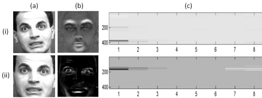
Fig. 5. Effect of alignment. Shown for C-HiSLR with \tau_{trn} = 4 . (a) is the test input ( fear ). (b) and (c) are recovered DX and X , respectively. (i) is under imperfect alignment while (ii) is under perfect alignment. X in (i) is not group-sparse.
