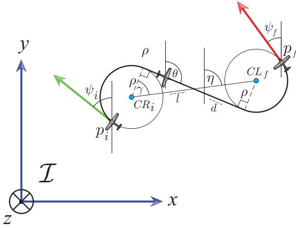
Fig. 5. Right-Straight-Left (RSL) Dubins path.
