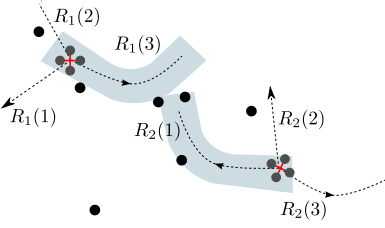
Fig. 3. At the start of each round, we have a set of m candidate trajectories per robot. The trajectories may be non-uniform and of varying speeds. Using the predicted motion of the targets, we can determine which targets will be covered for a given trajectory and the corresponding quality of tracking.
