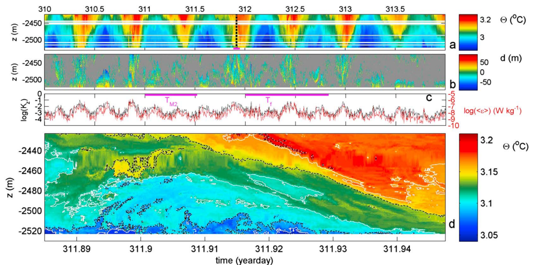
Figure 4. As Figure 3, but for site B. (a) Missing sensor data are indicated by horizontal bands. These are linearly interpolated for further analysis. (d) Dashed black contours are drawn every 0.05^\circ\text{C} , solid white every 0.025^\circ\text{C} . Note change in color scales for Figures 4a and 4d.
