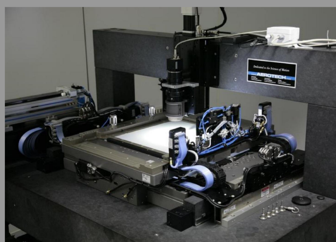
Sub-micrometric ROB digitizer
