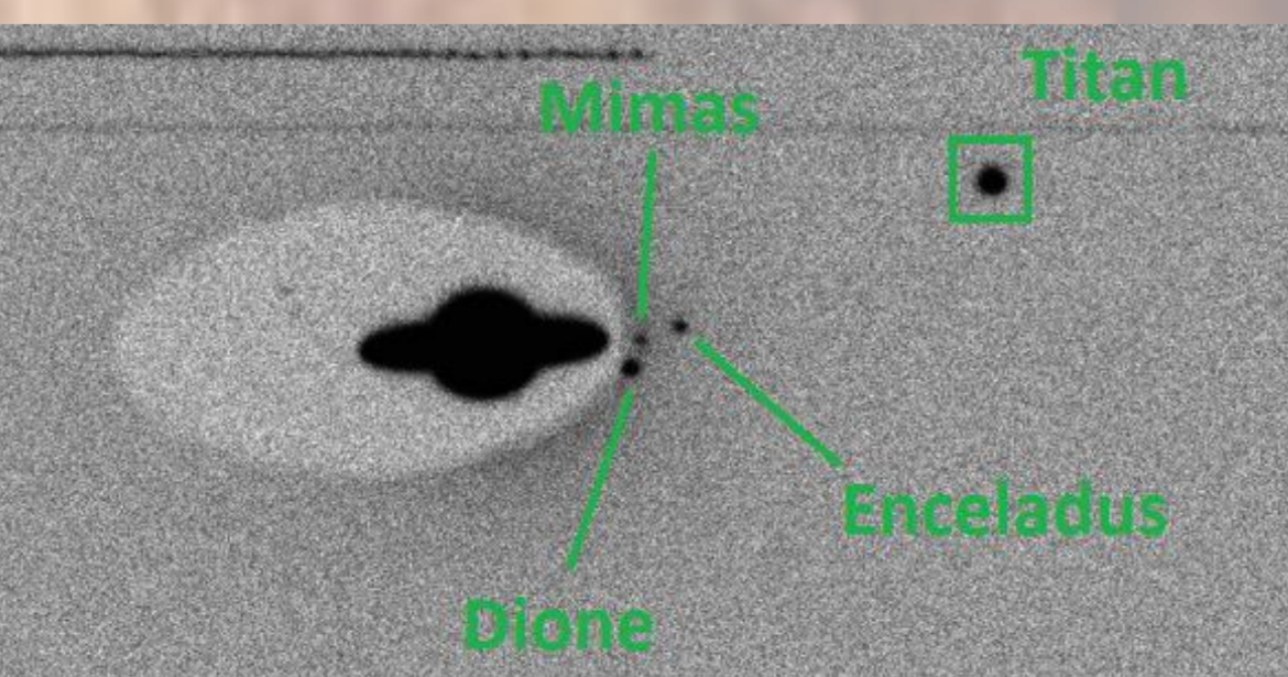
The USNO Saturnian plate n°23005 and center
