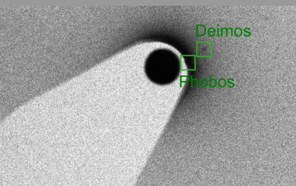
The USNO Martian plate n°11001 and center
