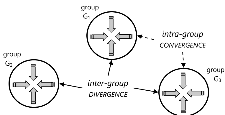
Figure 12 – Global divergence results from events of local convergence: Individual speakers adopt local innovations within their social network, thereby increasing the gap with neighbouring groups
