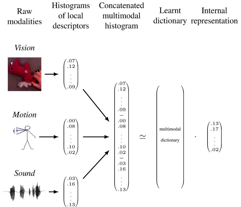
Fig 4. The MCA-NMF system processing of data. First raw data from each modality is transformed into a histogram of local descriptors, that is a vector of nonnegative values. Then the histograms from each modality are concatenated into a histogram representation of the multimodal perception. During its training the MCA-NMF system uses a set of perceived example, each represented by such an histogram, to learn a multimodal dictionary that captures multimodal patterns. The system then uses the dictionary to transform perception into an internal representation. The internal representation can be obtained with all modalities observed (as on the figure) or with only a subset of modalities observed as explained further.
