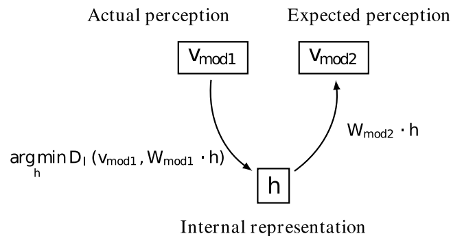
Fig 5. Once the system has learnt the dictionary ( W_{mod1} and W_{mod2} ), given an observation v_{mod1} in one modality it can reconstruct the corresponding internal representation as well as the expected perception in another modality.
