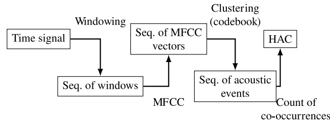
Fig 9. Sequence of transformations from raw (time sequence) acoustic signal to histograms of acoustic co-occurrence (HAC) representation.
