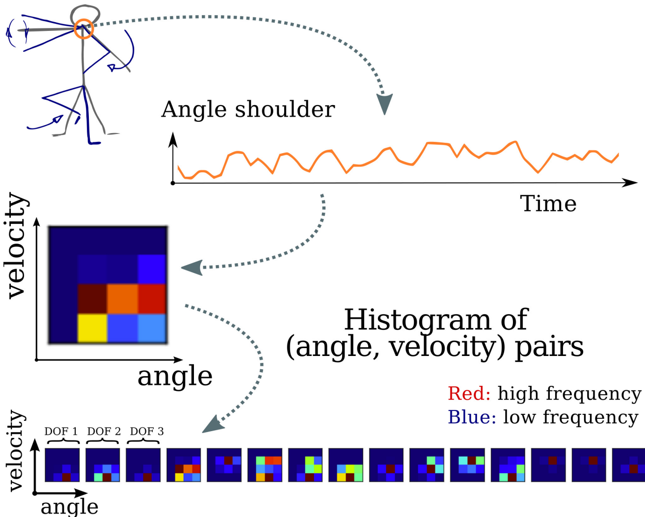
Fig 8. Human motions are abstracted as concatenated histograms on joint positions and velocities. In the final histograms, frequencies are represented through colors, x and y axis correspond respectively to values of angles and velocities. (Best seen in color.)
