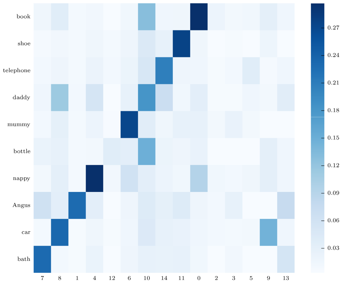
Fig 14. Some components are more associated with some semantic labels. The figure represents the mutual information between (vertically) semantic classes (that are not observed by the learner) and (horizontally) each internal set coefficient used by the learner to represent joint occurrences of motion demonstrations, object images, and acoustic descriptions from the training set. A value of k = 15 was used in this experiment.
