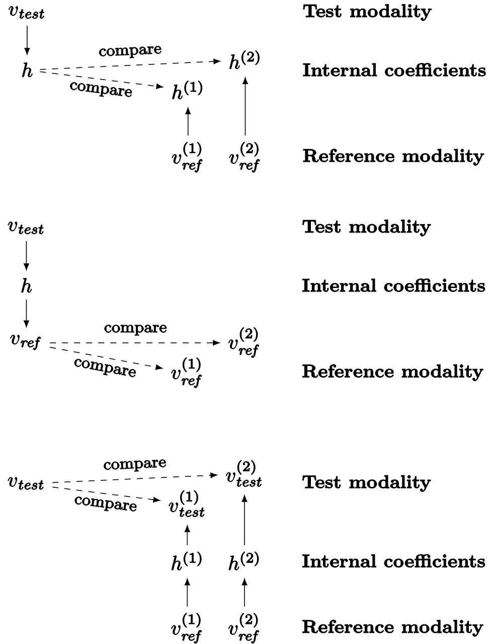
Fig 7. The multimodal classification task may be implemented as three different comparisons by MCA-NMF. On top, internal coefficients computed from the test example are compared to those computed from each reference example. In the middle, an expected representation of the test example in the reference modality is computed. Then this representation is compared to the actual perceptions of reference examples. Finally at the bottom, expected representations of the reference examples in the test modality are computed and compared to the actual perception of the test example.
