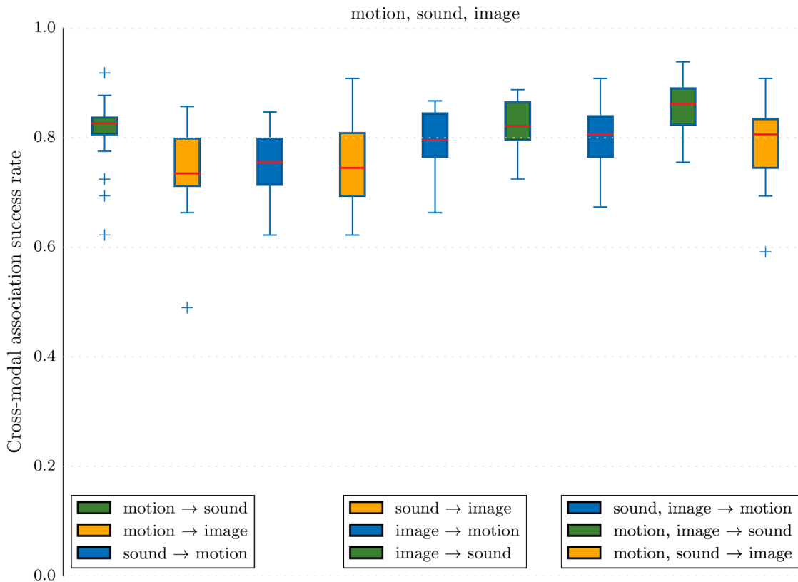
Fig 12. MCA-NMF is capable of relating information from many modalities to one. There is however no substantial improvement in performance from the use of two modalities as input for the recognition. The figure presents box plots of classification success rates for various experiments where three modalities are used for training. There are boxes representing the average success as well as quantiles and extreme values through cross-validation for various testing setups.
