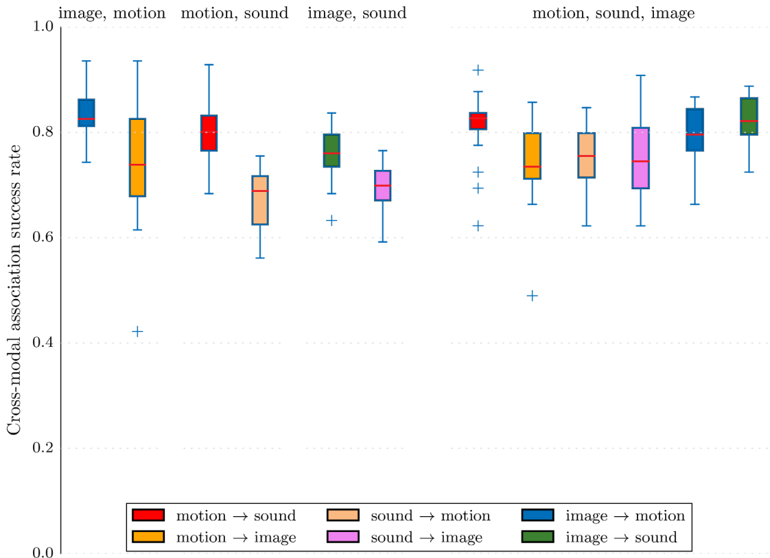
Fig 10. An additional modality during training slightly improves results in average. The box plot represents classification success rates for various experiments where two or three modalities are used for training. Each plot corresponds to the use of a subset of modalities during training: the first three plots use two modalities and the last one use three modalities. Each plot contains boxes representing the average success as well as quantiles and extreme values through cross-validation for various testing setups of the form A \rightarrow B . There are only two testing setups when only two modalities are used for training, and six when three modalities are used for training.
