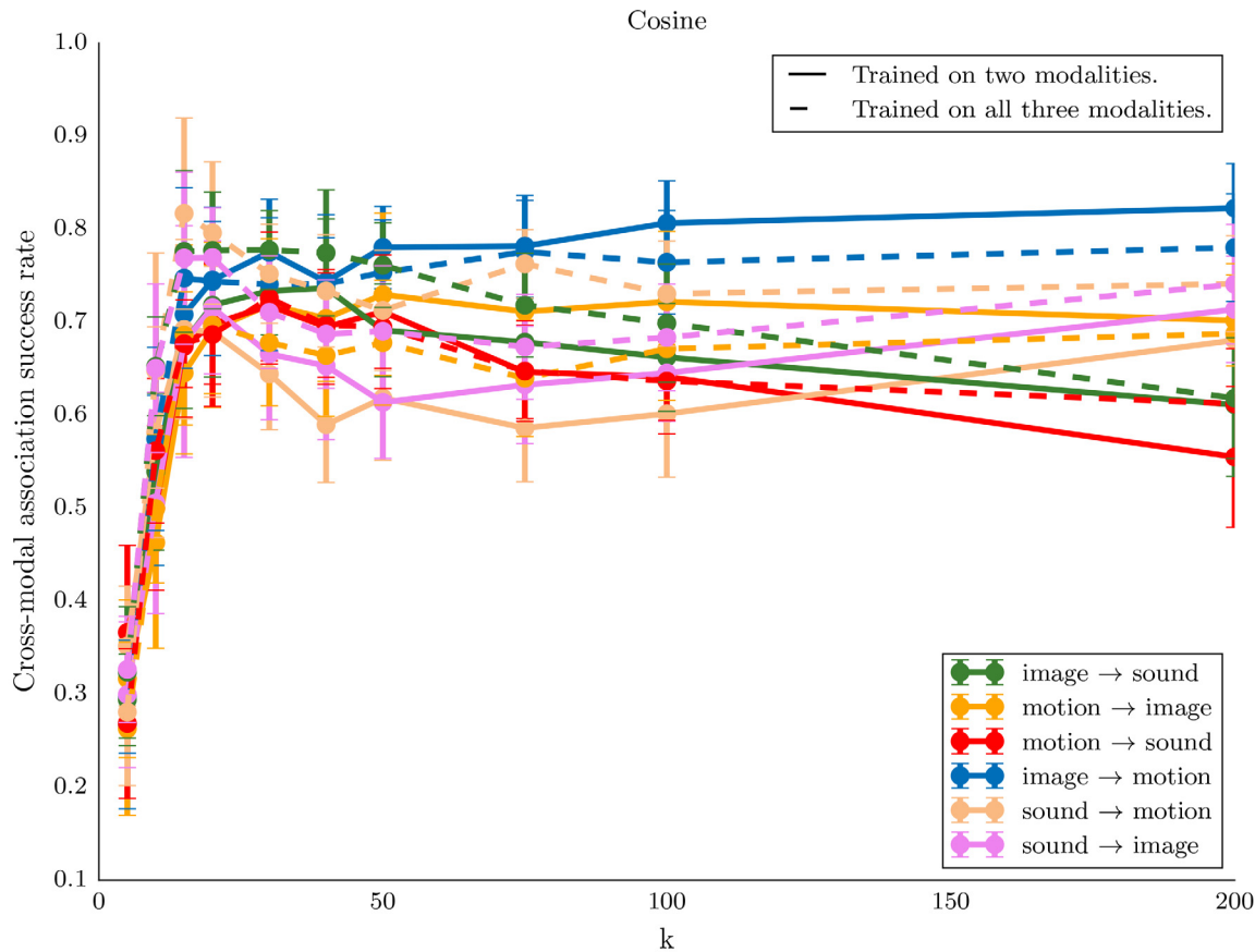
Fig 11. With both two (full lines) and three (dashed) modalities during training, the classification success rates are similar and good for high enough value of the number k of elements in the NMF dictionary. The plots demonstrate that the success rate is quite stable above a minimum value of k .
