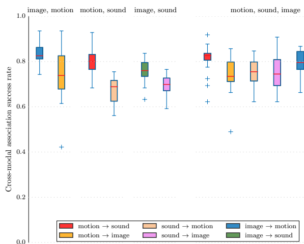
Fig. 9. An additional modality during training does not significantly impact result. The box plot represent classification success rates for various experiments where two or three modalities are used for training. Each plot corresponds to the use of a subset of modalities during training: the first three plots use two modalities and the last one use three modalities. Each plot contains boxes representing the average success as well as quantiles and extreme values through cross-validation for various testing setups, using only two modalities. There are only two testing setups when only two modalities are used for training, and six when three modalities are used for training.
