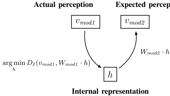
Fig. 5. Once the system has learnt the dictionary ( W_{mod1} and W_{mod2} ), given an observation v_{mod1} in one modality it can reconstruct the corresponding internal representation as well as the expected perception in another modality.
