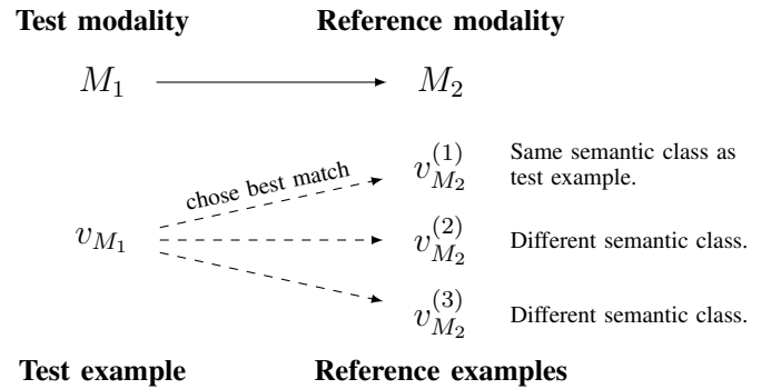
Fig. 6. The learner is tested on its ability to relate an observation of a test example in one modality to the right reference example in another modality.
