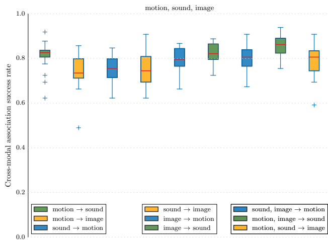
Fig. 11. MCA-NMF is capable of relating information from many modalities to one. There is however no substantial improvement in performance from the use of two modalities as input for the recognition. The figure presents box plots of classification success rates for various experiments where three modalities are used for training. There are boxes representing the average success as well as quantiles and extreme values through cross-validation for various testing setups.
