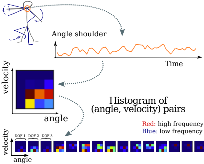
Fig. 7. Human motions are abstracted as concatenated histograms on joint position and velocities. In the final histograms, frequencies are represented through colors, x and y axis correspond respectively to values of angles and velocities. (Best seen in color)
