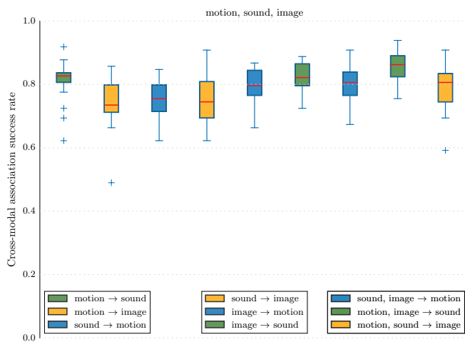
Fig. 10. MCA-NMF is capable of relating information from many modalities to one. There is however no substantial improvement in performance from the use of two modalities as input for the recognition. The figure presents box plots of classification success rates for various experiments where three modalities are used for training. There are boxes representing the average success as well as quantiles and extreme values through cross-validation for various testing setups.
