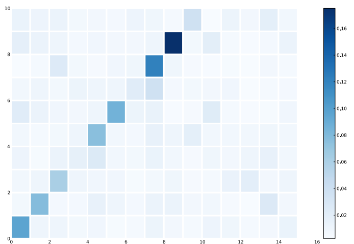
Fig. 12. Some components are more associated with some semantic labels. The figure represents the mutual information between (vertically) semantic classes (that are not observed by the learner) and (horizontally) each internal coefficient used by the learner to represent pairs of motion demonstration and acoustic descriptions from the training set. A value of k = 15 was used in this experiment.
