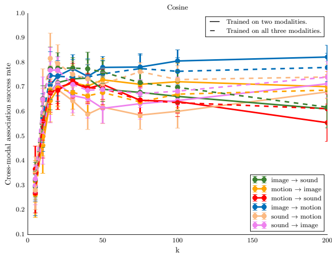
Fig. 9. With both two (full lines) and three (dashed) modalities during training, the classification success rates are similar and good for high enough value of the number k of elements in the NMF dictionary. The plots demonstrate that the success rate is quite stable above a minimum value of k .
