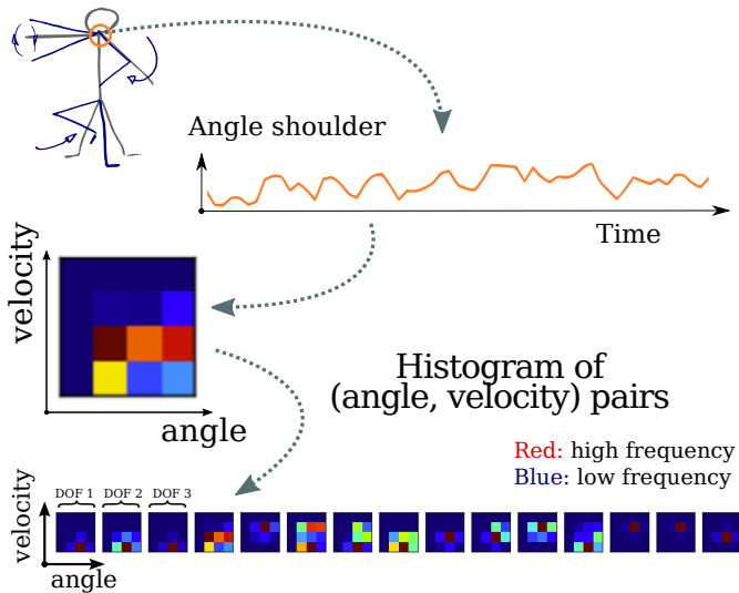
Fig. 6. Human motions are abstracted as concatenated histograms on joint position and velocities. In the final histograms, frequencies are represented through colors, x and y axis correspond respectively to values of angles and velocities. (Best seen in color)
