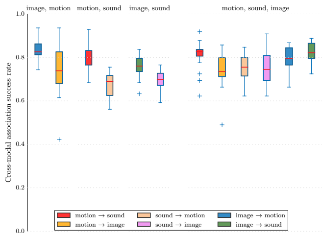
Fig. 8. An additional modality during training does not significantly impact result. The box plot represent classification success rates for various experiments where two or three modalities are used for training. Each plot corresponds to the use of a subset of modalities during training: the first three plots use two modalities and the last one use three modalities. Each plot contains boxes representing the average success as well as quantiles and extreme values through cross-validation for various testing setups, using only two modalities. There are only two testing setups when only two modalities are used for training, and six when three modalities are used for training.
