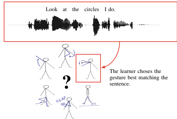
Fig. 1. Illustration of the cross-modal classification task on which one learner presented in this article is tested. The transcriptions of the spoken utterances are represented on the figure to illustrate the keyword semantics. However, in the experiments we present the learner does not observe these transcriptions.
