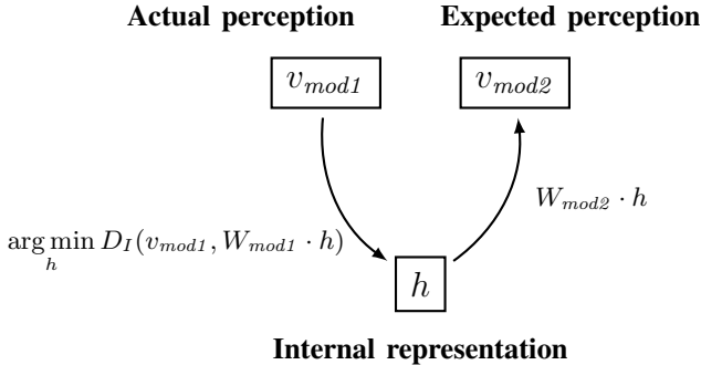
Fig. 4. Once the system has learnt the dictionary ( W_{mod1} and W_{mod2} ), given an observation v_{mod1} in one modality it can reconstruct the corresponding internal representation as well as the expected perception in another modality.
