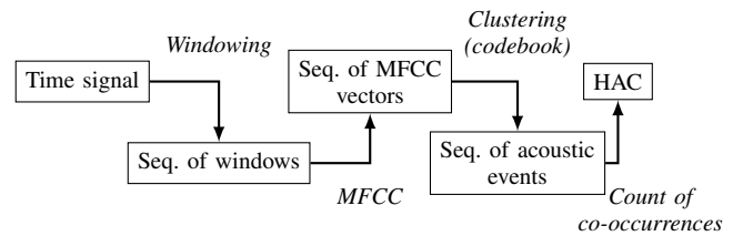
Fig. 7. Sequence of transformations from raw (time sequence) acoustic signal to histograms of acoustic co-occurrence (HAC) representation.
