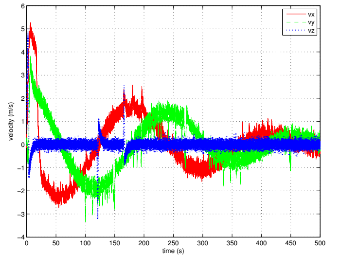
Fig. 4. Measured velocity.
