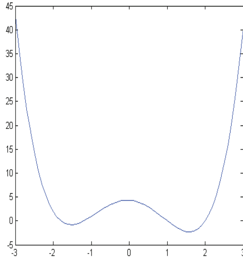
Figure 5: Graphical Solution of Example 3 with DCA
