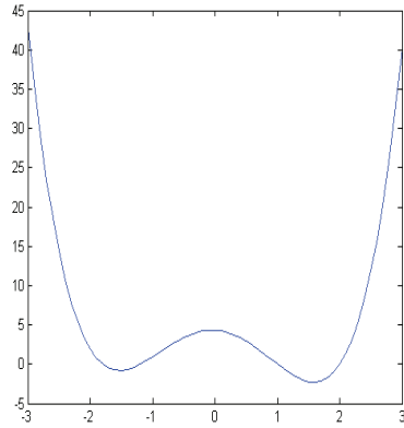
Figure 6: Solution of Example 4 (DCA) Figure 7: Solution of Example 4 (MDCA)
