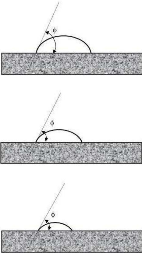
Fig. 6. Schematic evolution in time of the behavior of a drop in contact with a porous substrate showing the decrease of drop volume and contact angle.
