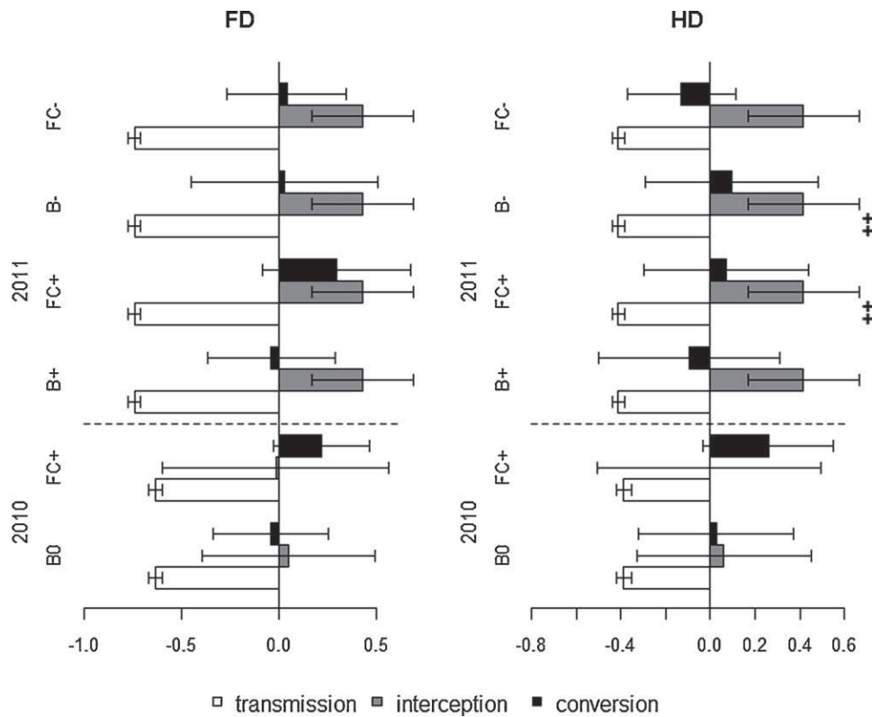
Fig. 6. Contribution of transmission, interception and conversion of light into biomass in FD and HD treatments. Horizontal bars represent log-relative efficiencies \log_{10}RTE , \log_{10}RIE , and \log_{10}RCE . Error bars feature standard deviation of respective efficiencies. '++' indicates varieties for which dry matter in HD exceeded dry matter in the full sun.
