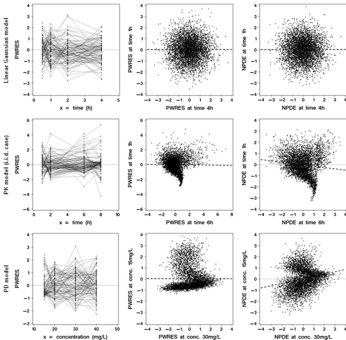
Fig. 6 Illustration of data dependency within subjects for the different models investigated: the linear Gaussian model ( top ), the population PK model ( middle ) and the population PD model ( bottom ). The graphs shows from left to right the plots of weighted residuals (PWRES) vs. the independent variable x , PWRES at one value of x vs. PWRES at another value of x , and NPDE at one value of x vs. NPDE at another value of x (the last two graphs were performed in 5,000 subjects instead of 100 to clearly illustrate data dependency). The dashed line refers to a linear regression line through the data. A horizontal dashed line indicates that the data are uncorrelated. A rounded shape for the data indicates that the data are independent.
