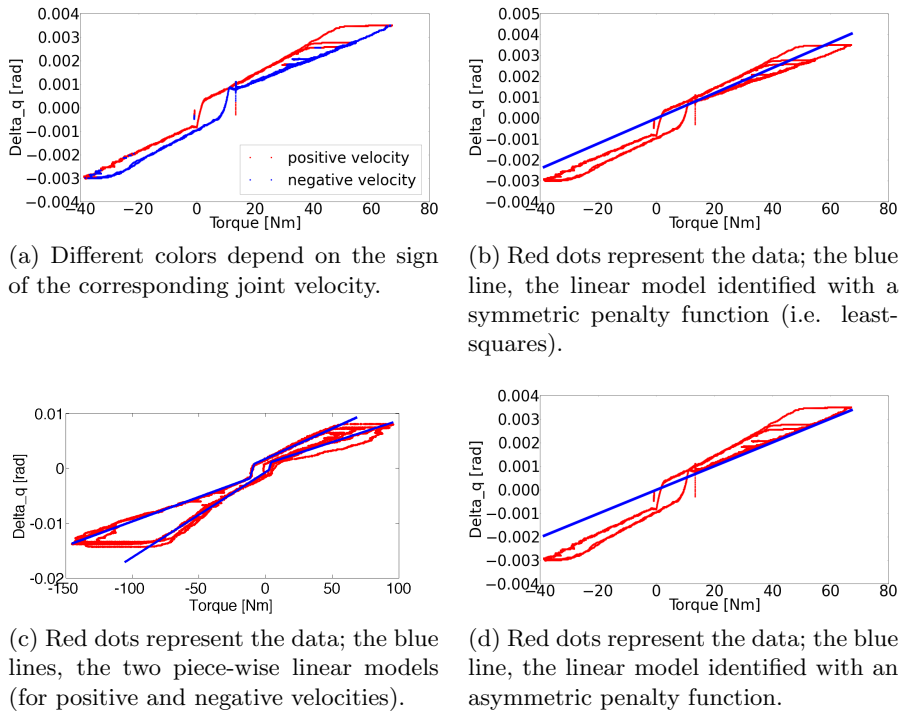
Figure 1: Torque \tau vs. position error \Delta_q for the right knee (a, b, d) and right hip-pitch (c) joints of HRP-2. These data have been collected on one position-controlled joint keeping q_j^d constant and applying external forces. The joint is nearly static, so that \dot{q}_j \approx 0 . From (6), we expect \Delta_q = K_\tau \tau , but the data clearly do not fit.
