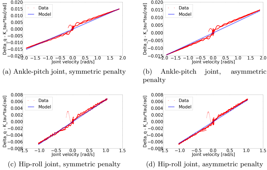
Figure 3: Friction identification: comparison of the two penalty functions: [left] symmetric penalty (7) [right] asymmetric penalty (8). Each plot displays the friction part of the model ( \Delta_q - K_\tau\tau ) wrt the velocity ( \dot{q}_j ). The data have been collected tracking a sinusoidal reference with increasing amplitude. The symmetric penalty tends to overestimate the friction, while the asymmetric penalty mostly underestimates while keeping a fit of similar quality.
