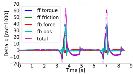
(d) Knee joint, inverse-dynamics control with K_6 = 1 .
