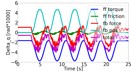
(f) Ankle-pitch joint, force control.
