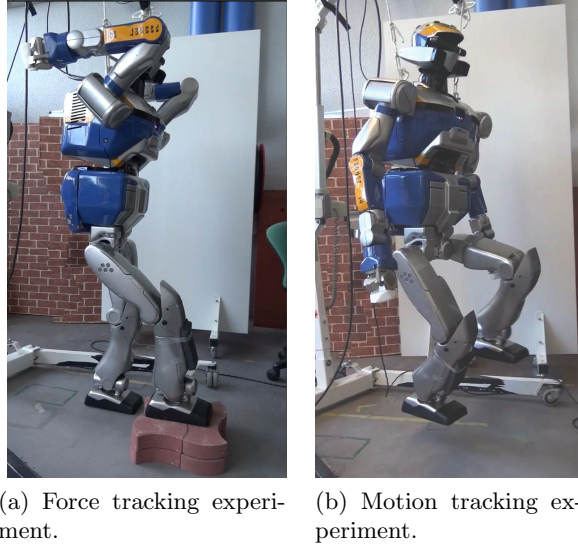
Figure 2: Experimental setup.
