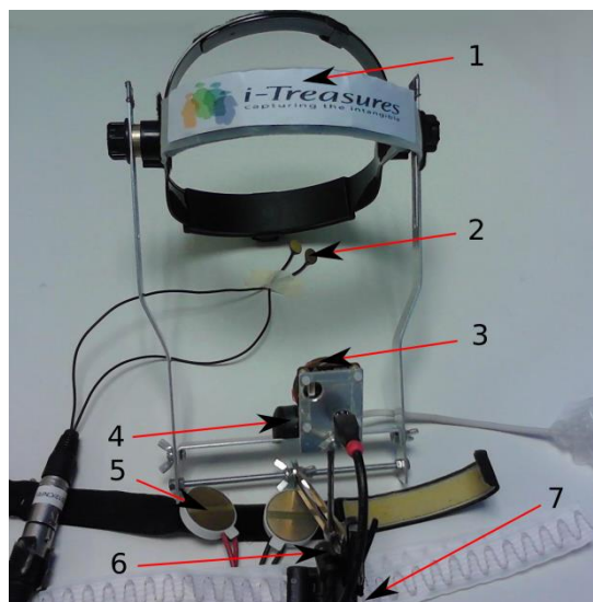
Figure 1. Acquisition sensors.
