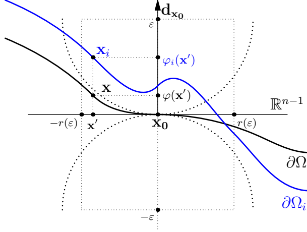
Figure 2: Illustration of Theorem 3.3 stating that there exists a fixed common local frame in which a converging sequence of elements in \mathcal{O}_\varepsilon(B) can be simultaneously parametrized by C^{1,1} -graphs.
