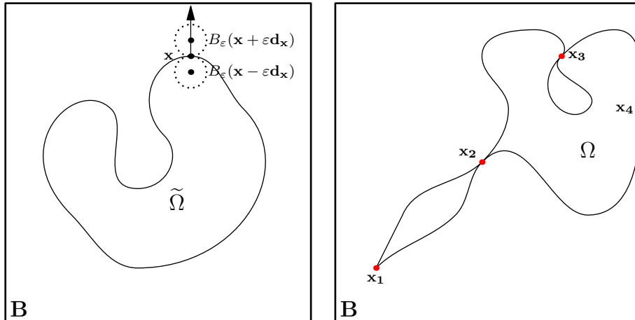
Figure 1: Example of an open set \tilde{\Omega} \subset B satisfying the \varepsilon -ball condition whereas \Omega \subset B does not. Indeed, there is no circle passing through the points \mathbf{x}_1 and \mathbf{x}_2 (respectively \mathbf{x}_3 and \mathbf{x}_4 ) whose inner domains are included in \Omega (respectively in B \setminus \Omega ).
