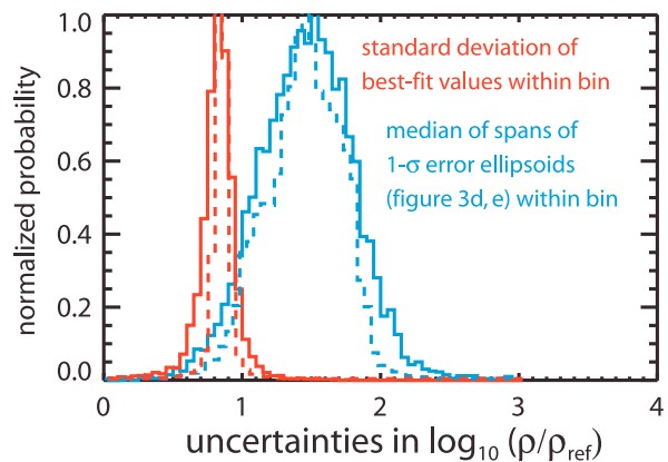
Figure 7. A priori and a posteriori uncertainties across the data set. The red lines are histograms of the standard deviation of values of \log_{10}[\rho/\rho_{\text{ref}}] within each bin of latitude and Ls, i.e., an a posteriori measure of uncertainty. The blue lines are histograms of the median of spans in \log_{10}[\rho/\rho_{\text{ref}}] of 1\text{-}\sigma error ellipsoids (i.e., twice the a priori estimate of uncertainty) within the same bins. Solid lines represent unsmoothed bin sizes of 5^\circ in latitude and 5^\circ in Ls. Dashed lines represent boxcar-smoothed bins of 15^\circ in latitude and 25^\circ in Ls.
