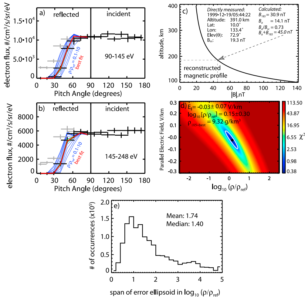
Figure 3. Fit to a typical loss cone. (a and b) Typical electron loss cones measured at 1999-12-19/05:44:22 in two adjacent energy channels. The incident and reflected (i.e., down- and up-traveling) flux are on the right and left, respectively. The flux measurements before backscatter subtraction are shown in gray, while those after are shown in black. The best fit to the loss cone is shown in red, while the predicted loss cone shapes for values of \rho/\rho_{\text{ref}} (i.e., the ratio between mass density and a reference density, see text) between 0.1 and 10 are shown in blue. (c) The most likely magnetic field profile used in calculating the predicted loss cones (see text in section 2.2). (d) The \chi^2 landscape for this particular fit with the 1- \sigma error ellipsoid shown in white. \rho_{185} refers to the best estimate of the mass density at 185 km derived from this particular loss cone. (e) The distribution of the span of the error ellipsoid in \log_{10}\rho/\rho_{\text{ref}} over the entire usable data set (i.e., including only data points with magnetic elevation angles greater than 40^\circ and values of B_{185} greater than 15 nT, as discussed in section 3.1).
