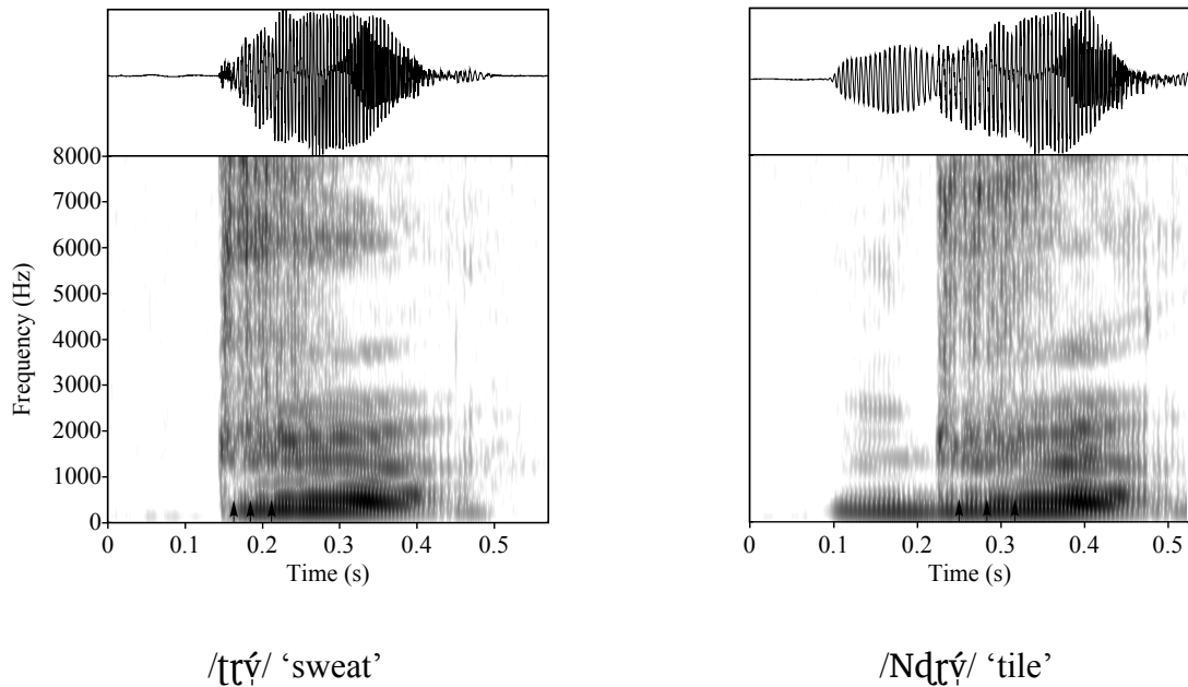
Figure 6: Waveforms and spectrograms of /tʁʏ/ ‘sweat’ and /Ndʁʏ/ ‘tile’ (arrows indicate contacts between the tip of the tongue and the roof of the mouth)
