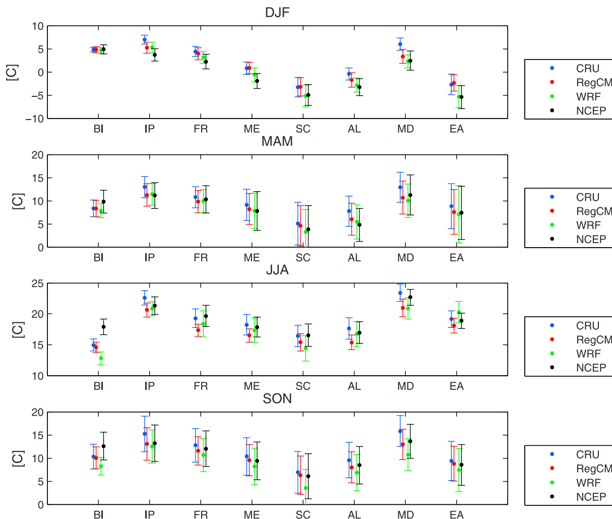
Figure 2. Seasonal mean (2002–2006) values of observed (CRU, blue), reanalyzed (NCEP, black), and simulated (RegCM3, red, WRF, green) 2 m temperature over the eight European PRUDENCE subregions with the associated standard deviations. Only the land data are included in the regional average. (top to bottom) Winter, spring, summer, and fall.
