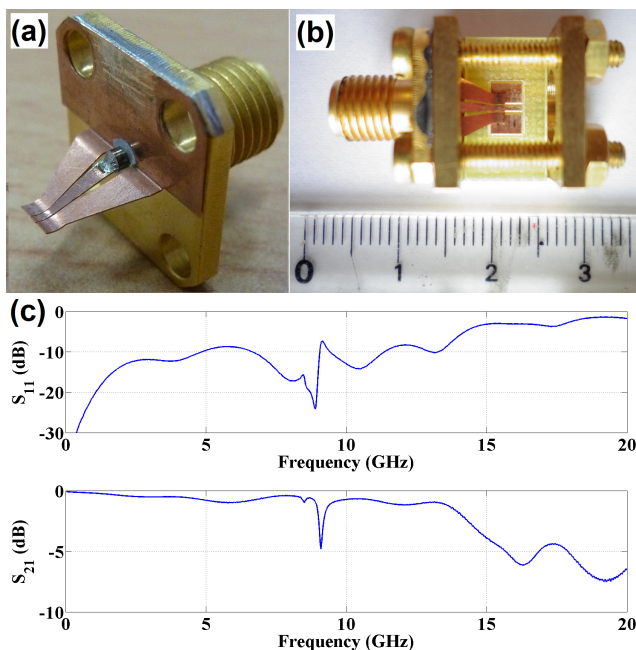
Fig. 1. a) Copper-beryllium probe on its SMA connector. The tapering from the connector to the tip of the tongs is linear. b) Setup for HF characterization of the probes; only one is present in order to show the underlying copper strips. c) S_{11} and S_{21} measurements of the contacting probes describing reflection and transmission properties of the device.
