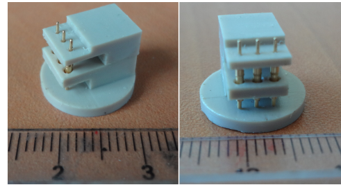
Fig. 4. Sample holder for synchrotron experiments with mounted spring-loaded contacts. The CPW is laid on the top flat surface and held in place by a metallic cap (not shown here) belonging to the microscope optics.
