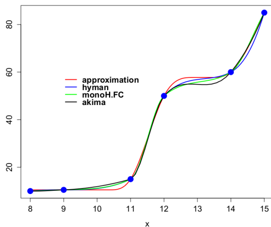
Fig. 12: Monotone cubic splines interpolation for four different methods using Akima's data.
