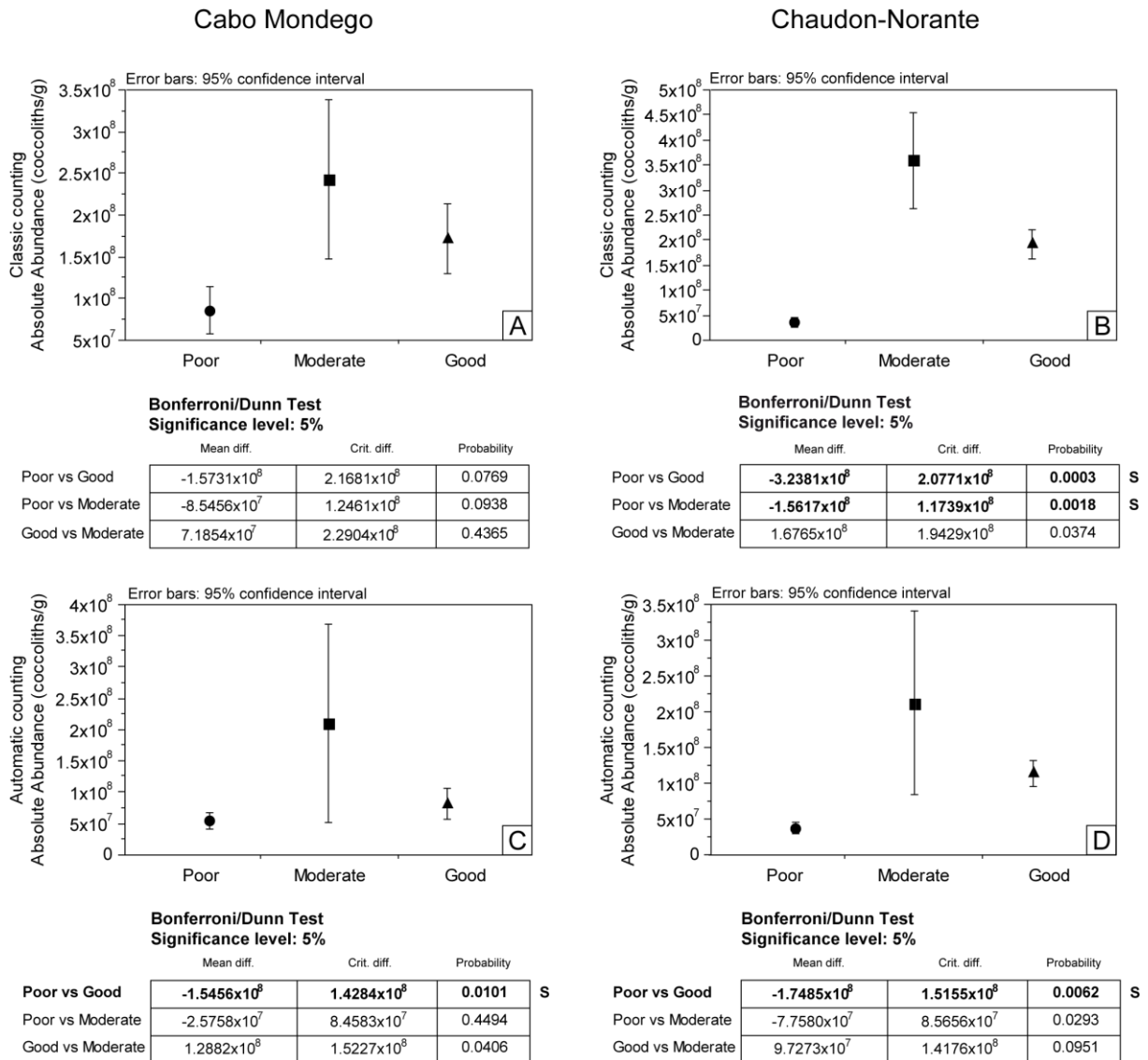
Figure 7: Bonferroni/Dunn test between preservation states and classic counting of absolute abundances at Cabo Mondego (A) and Chaudon-Norante (B), and between preservation states and automatic counting of absolute abundances at Cabo Mondego (C) and Chaudon-Norante (D).
