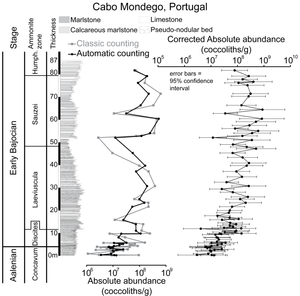
Figure 2: Stratigraphic variations of absolute abundance calculated based on automatic counting (black circles) and classic counting (gray squares) at Cabo Mondego. The corrected absolute abundance for all automatic counting samples is based on correlation regression. Error bars have been calculated based on the 95% confident band for the fitted correlation regression (see also Fig. 4).
