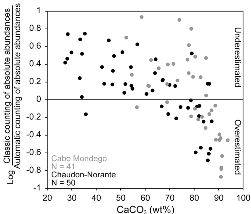
Figure 8: Plot of \text{wt}\%\text{CaCO}_3 versus the log ratio of classic counting/automatic counting of absolute abundances. Samples from Cabo Mondego are represented in gray and those from Chaudon-Norante in black. The log of the ratio was taken in order to center the data around 0, where 0 represents no difference between classic and automatic counting methods. SYRACO underestimated samples are found between 0 and 1, whereas overestimated samples are found between -1 and 0.
