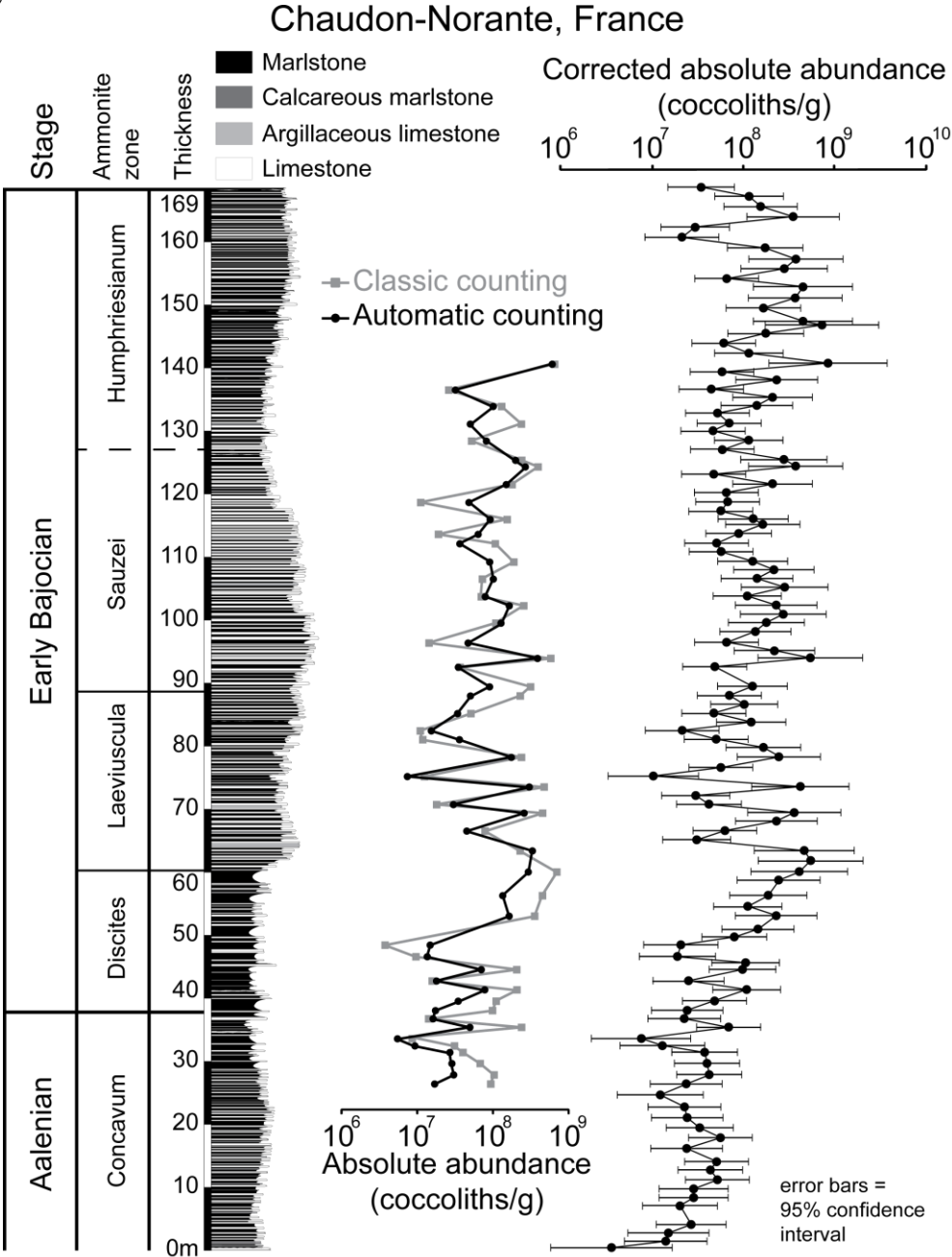
Figure 3: Stratigraphic variations of absolute abundance calculated based on automatic counting (black circles) and classic counting (gray squares) at Chaudon-Norante. The corrected absolute abundance for all automatic counting samples is based on correlation regression. Error bars have been calculated based on the 95% confident band for the fitted correlation regression (see also Fig. 4).
