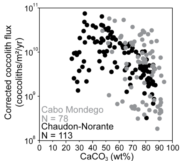
Figure 6: Plot of wt%CaCO 3 versus corrected coccolith flux (coccoliths/m 2 /year). Samples from Cabo Mondego are represented in gray and those from Chaudon-Norante in black.
