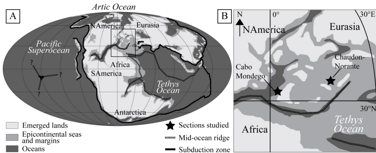
Figure 1: Paleogeographic map of the Middle Jurassic (after Blakey, 2008). On the left (A), a global view with subduction zones and mid-ocean ridges; and on the right (B), a focus on the western Tethys with the location of the Cabo Mondego section in the Lusitanian Basin.
