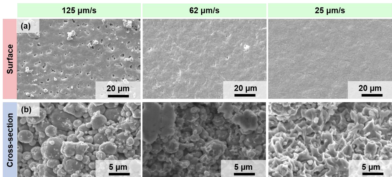
Figure 4. SEM micrographs of Cu sample surface fabricated by LS at different scan speeds:
