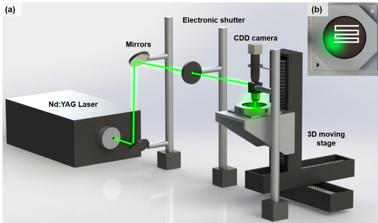
Figure 2. (a) Schematic of the homemade LS system and (b) line scanning strategy of the laser.
