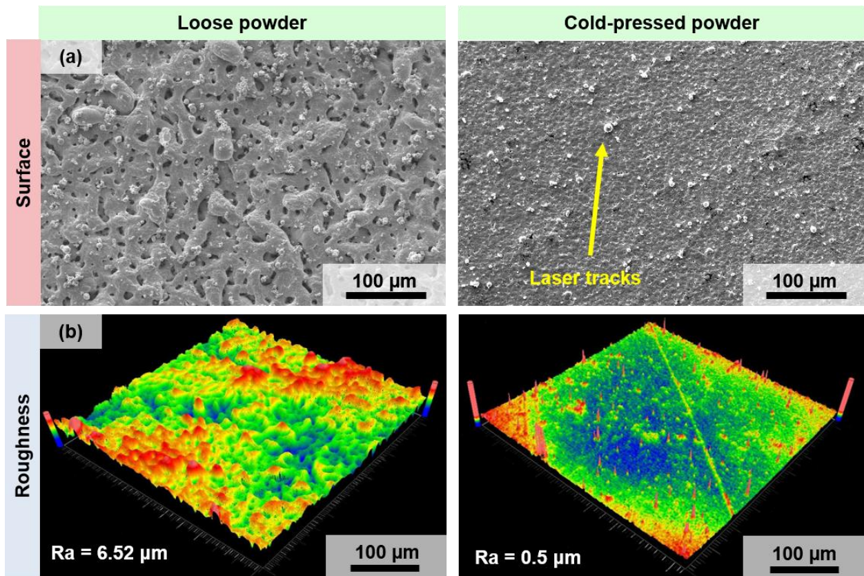
Figure 3. (a) SEM micrographs and (b) 3D surface mapping of Cu layer fabricated using LS from loose and cold-pressed Cu powders, respectively.
