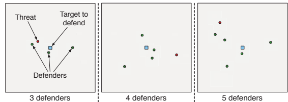
Figure 3: Example of system adaptation to the team size: the same GRN is used to handle teams composed of 3, 4 or 5 defenders. The team splits the environment according to the team size.
