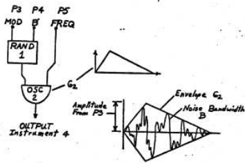
Fig 6 Noise Instrument
