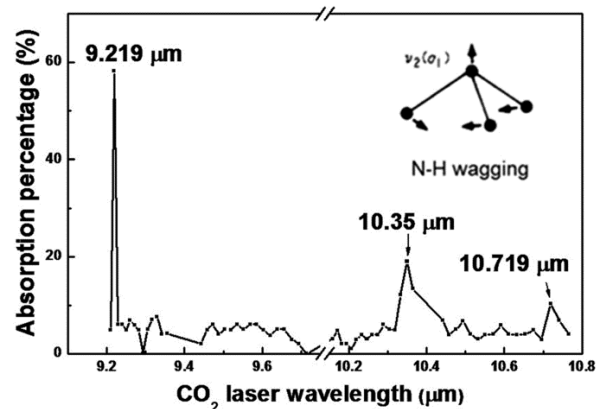
Figure 12. Absorption spectrum of the \text{CO}_2 laser power by \text{NH}_3 gas as a function of wavelength.
