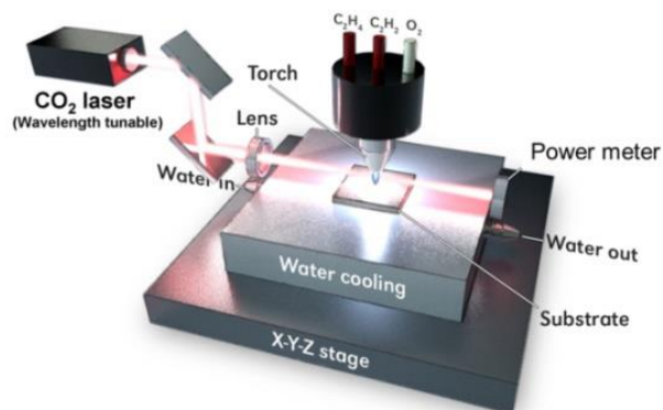
Figure 1. A schematic experimental setup of the LA-CCVD system.
