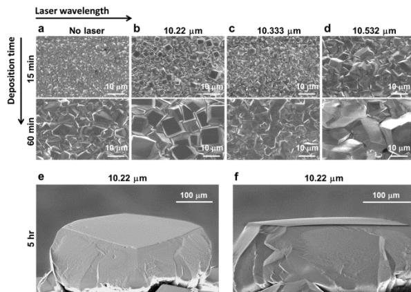
Figure 10. SEM micrographs of the diamond films and particles. (a-d) diamond films deposited without laser (a), with laser irradiation at 10.22 \mu\text{m} (b), 10.333 \mu\text{m} (c), and 10.532 (d). (e) and (f) single-crystal diamond grown with laser irradiation at 10.22 \mu\text{m} .
