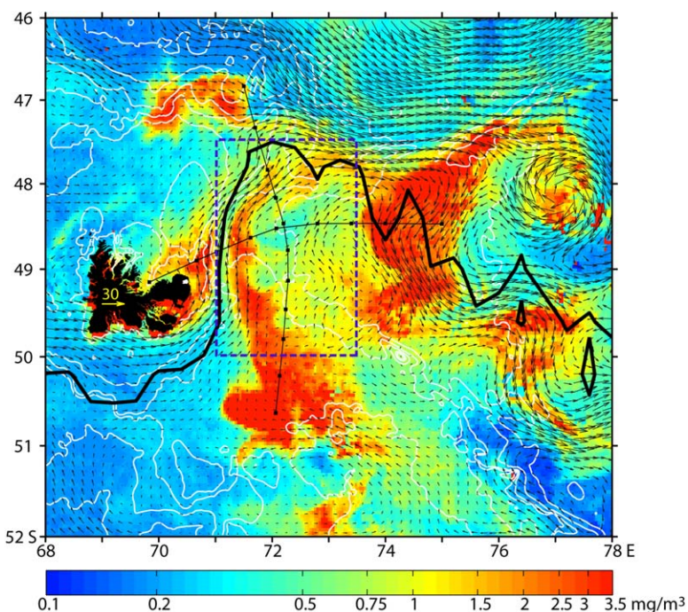
Figure 6. Mean surface velocity field during the KEOPS2 cruise constructed from the combined data sets of drifter-derived currents within the dashed rectangular area and altimeter-derived currents outside the rectangular area. The velocity scale for 30 \text{ cm s}^{-1} is shown on the Kerguelen Islands. See the text for the details of the methodology. Composite chlorophyll images (color shading) during the KEOPS2 cruise, the two transects (thin lines), and the PF_Park (thick black line) from Figure 5 are superimposed.
