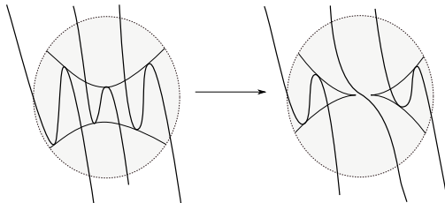
FIGURE 3. Generating family for the Lagrangian immersion.
