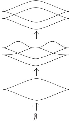
FIGURE 4. An exact filling of the Hopf link.
