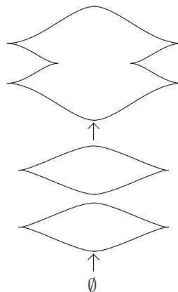
FIGURE 5. Movie of a Lagrangian immersion with a single double point.
