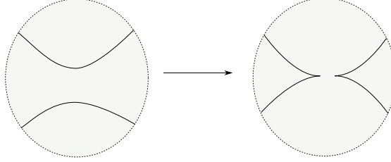
FIGURE 2. Local move realisable by a Lagrangian immersion.
