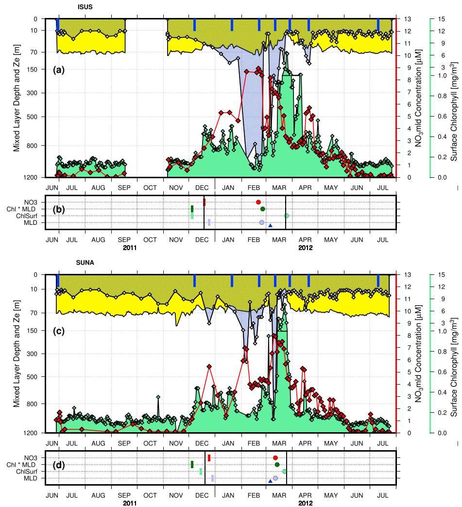
Figure 1. Time series and metrics of the PRONUTS and satellite observations for the (a and b) ISUS and for the (c and d) SUNA. In Figures 1a and 1c, grey diamonds represent MLD, red diamonds NO_{3mid} , yellow points Ze, and green diamonds CHL. The blue marks on the upper x axis of Figures 1a and 1c indicate the date of the satellite images drawn in Figure 2. In Figures 1b and 1d, vertical short colored lines indicate the dates of parameter increasing (red for NO_3 , dark green for CHL \times MLD , light green for CHL, and grey for MLD); circles indicate date of absolute maximum (same color code); and black lines indicate the dates of the first and the last occurrences of the MLD = Ze condition. Triangles indicate the date of negative-to-positive Qtot inversion. See Table S2 in the supporting information for the list of the metric values and of the method to compute them.
