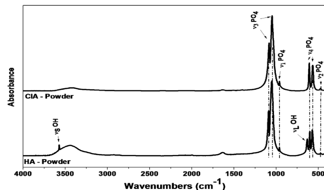
Fig. (2). FTIR spectra of the HA and CIA powders used in this work. Apatitic phosphate absorption bands are indicated by dotted lines.
