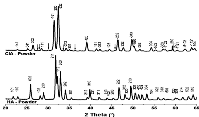
Fig. (1). Diffraction patterns of the HA and CIA powders used in this work. Superlattice lines on CIA pattern are shown by arrows.
