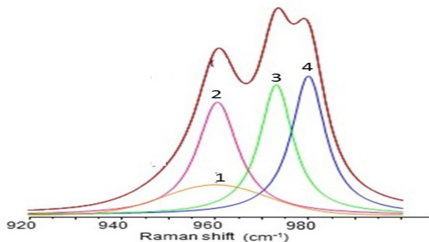
Fig. (10). A-Gaussian-Lorentzian curve fitting of the \nu_1\text{PO}_4 Raman stretching domain of HA coatings (20 spray runs), with the LEPS plasma gun. (1) ACP: amorphous calcium phosphate; (2) and (4) OA: oxyapatite; (3) HA: hydroxyapatite.
