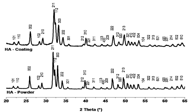
Fig. (4). X-ray diffraction patterns of HA powder and coating (12 spray runs).
