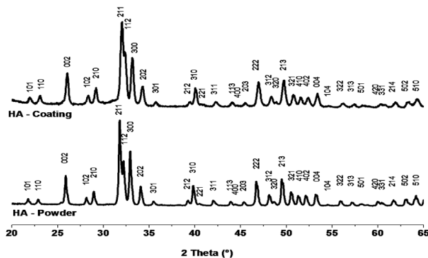
Fig. (5). X-ray diffraction patterns of CIA powder and coating (12 spray runs).
