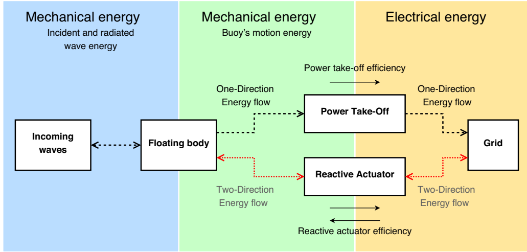
Fig. 2. Energy flow from the waves to the grid.
