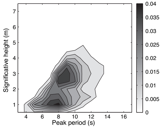
Fig. 7. Scatter diagram offshore the island of Yeu, France.
