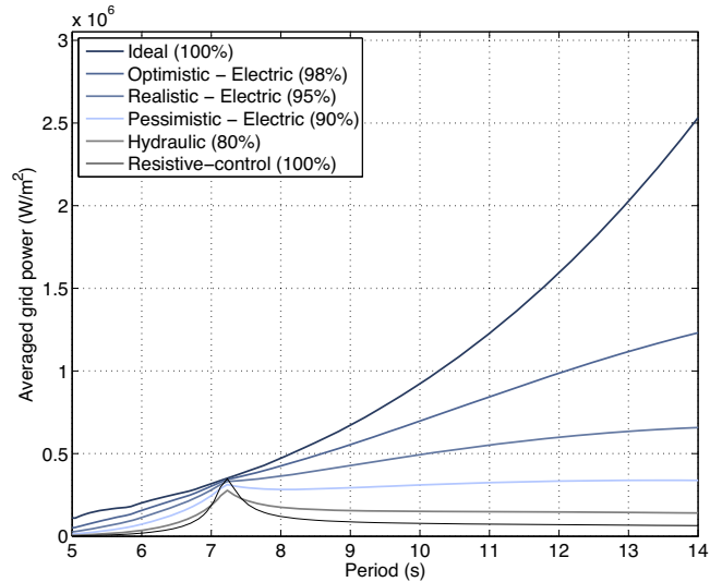
Fig. 5. Grid power as a function of wave period (regular waves) without control and with control with different actuators efficiencies.
