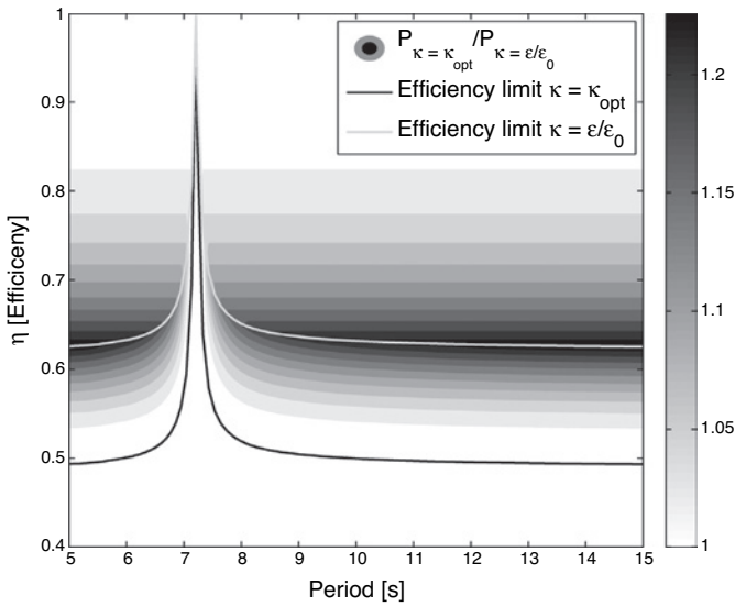
Fig. 3. Ratio between grid power with an optimal \kappa and grid power with \kappa = \epsilon/\epsilon_0 .
