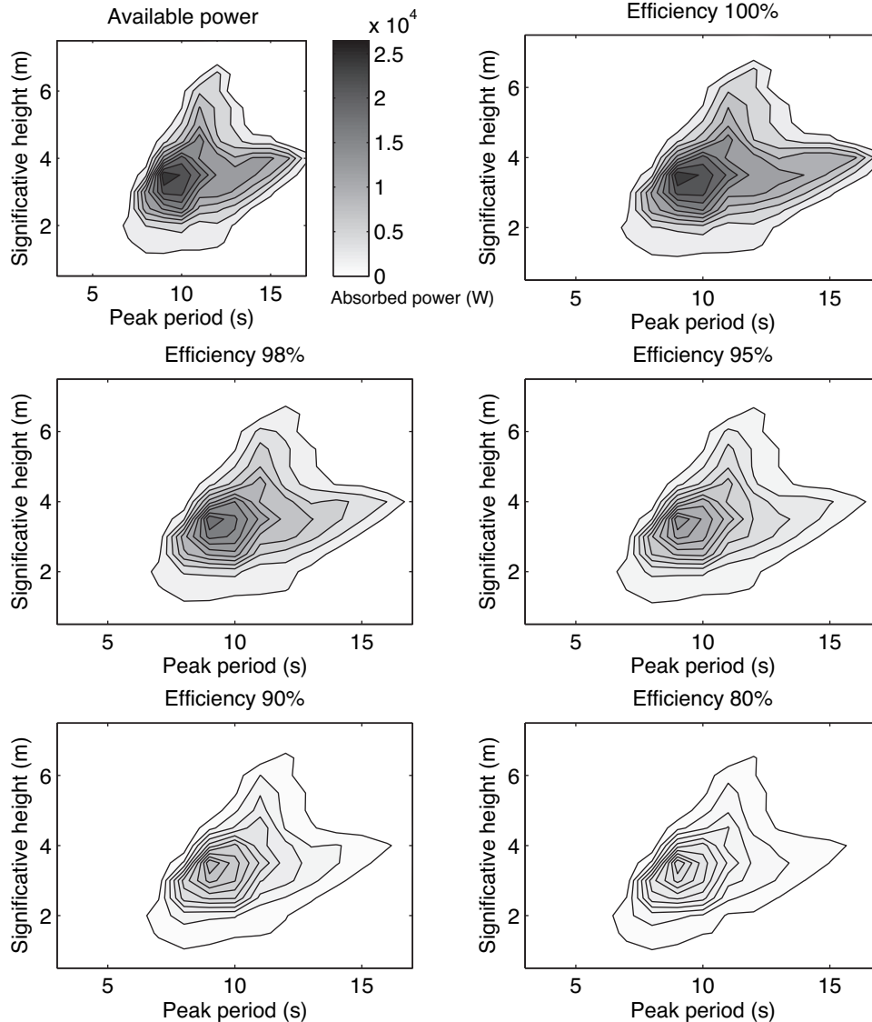
Fig. 8. Power matrices of the device with different actuators efficiencies.
