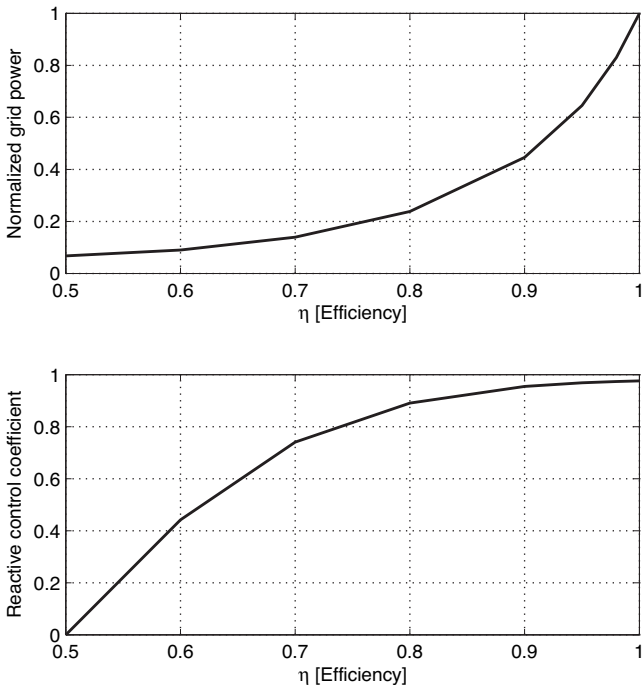
Fig. 4. Grid power and optimal reactive control coefficient as a function of actuators efficiency in a 9 s regular wave with 1 m wave amplitude.
