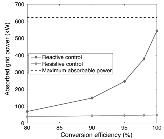
Fig. 9. Mean annual absorbed power at l'île d'Yeu under various conversion efficiency, France.
